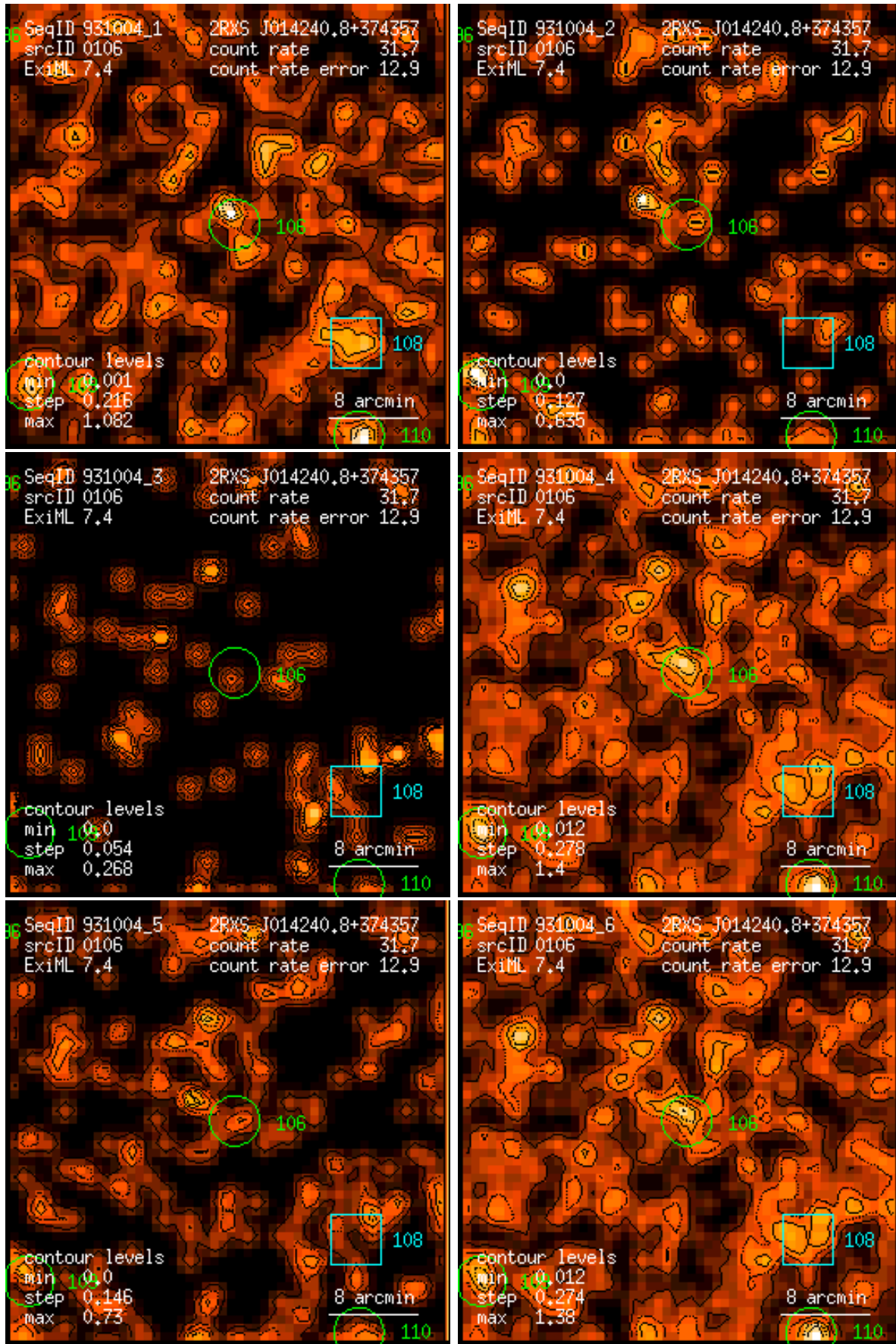
Figure 106: RASS 931004: detection 0106: band rate images, Gaussian filter: (1) PSPC channels 11 – 41, (2) 52 – 90, (3) 91 – 201, (4) 11 – 235, (5) 52 – 201, (6) 11 – 201. Broad band rates in counts/ks. Band rate contour levels in counts/ks/arcmin 2 .
