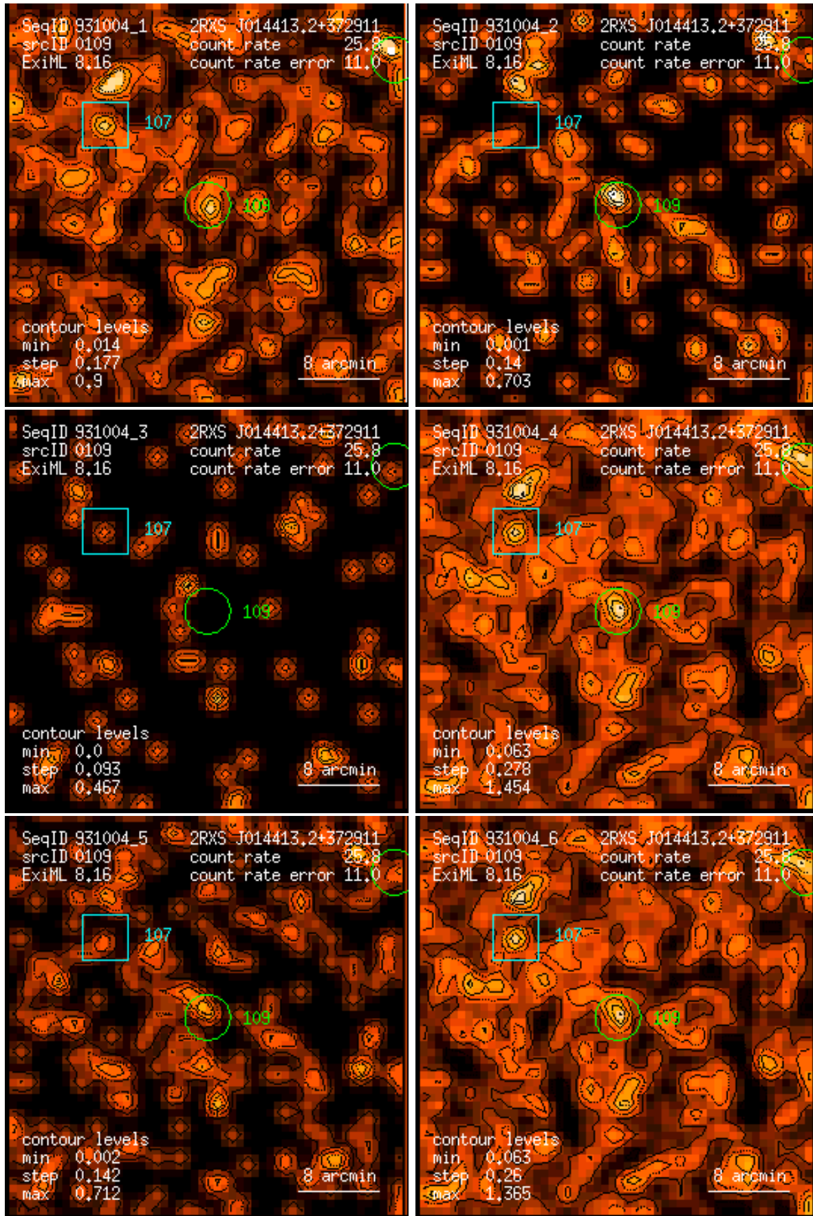
Figure 109: RASS 931004: detection 0109: band rate images, Gaussian filter: (1) PSPC channels 11 – 41, (2) 52 – 90, (3) 91 – 201, (4) 11 – 235, (5) 52 – 201, (6) 11 – 201. Broad band rates in counts/ks. Band rate contour levels in counts/ks/arcmin 2 .
