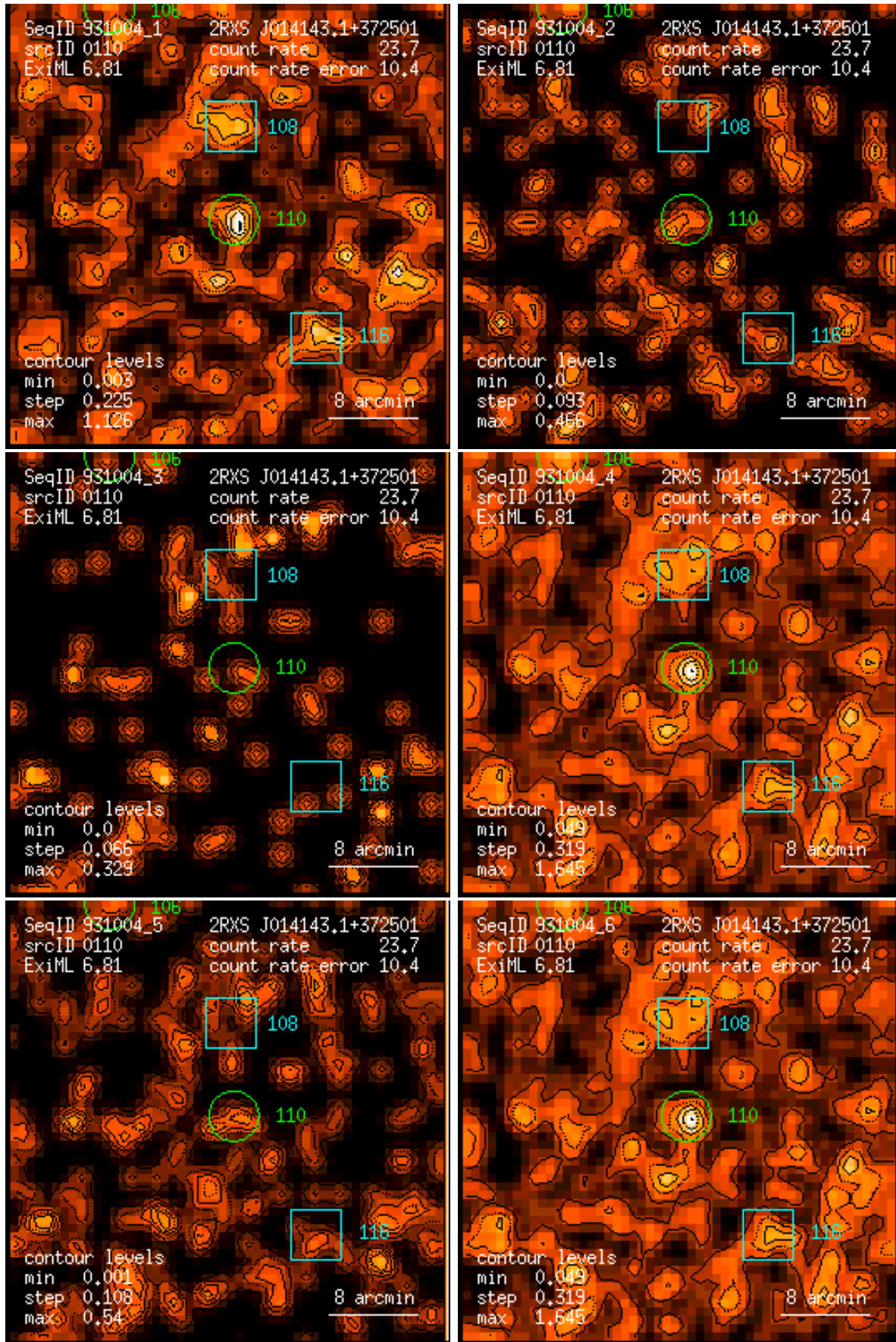
Figure 110: RASS 931004: detection 0110: band rate images, Gaussian filter: (1) PSPC channels 11 – 41, (2) 52 – 90, (3) 91 – 201, (4) 11 – 235, (5) 52 – 201, (6) 11 – 201. Broad band rates in counts/ks. Band rate contour levels in counts/ks/arcmin 2 .
