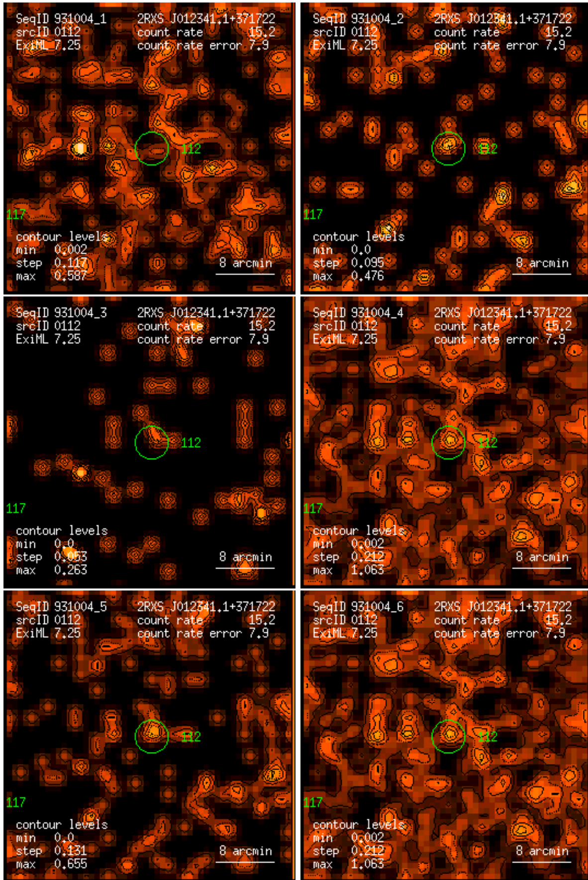
Figure 112: RASS 931004: detection 0112: band rate images, Gaussian filter: (1) PSPC channels 11 – 41, (2) 52 – 90, (3) 91 – 201, (4) 11 – 235, (5) 52 – 201, (6) 11 – 201. Broad band rates in counts/ks. Band rate contour levels in counts/ks/arcmin 2 .
