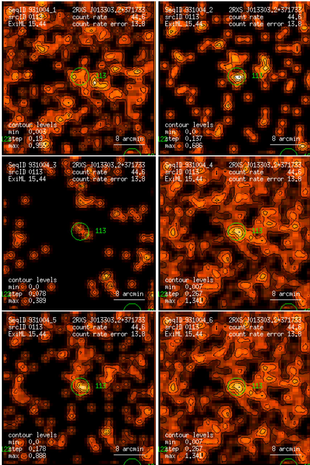
Figure 113: RASS 931004: detection 0113: band rate images, Gaussian filter: (1) PSPC channels 11 – 41, (2) 52 – 90, (3) 91 – 201, (4) 11 – 235, (5) 52 – 201, (6) 11 – 201. Broad band rates in counts/ks. Band rate contour levels in counts/ks/arcmin 2 .
