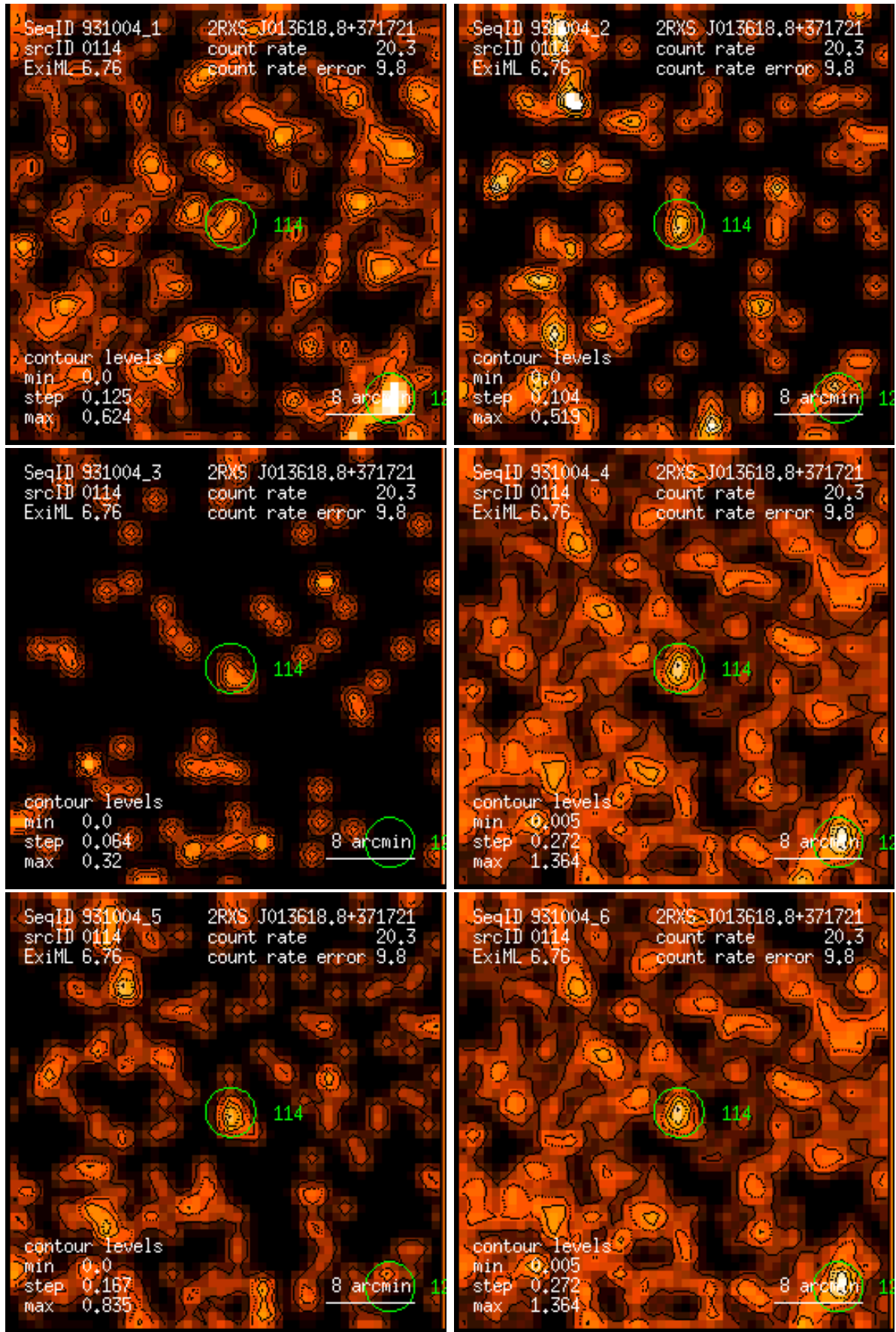
Figure 114: RASS 931004: detection 0114: band rate images, Gaussian filter: (1) PSPC channels 11 – 41, (2) 52 – 90, (3) 91 – 201, (4) 11 – 235, (5) 52 – 201, (6) 11 – 201. Broad band rates in counts/ks. Band rate contour levels in counts/ks/arcmin 2 .
