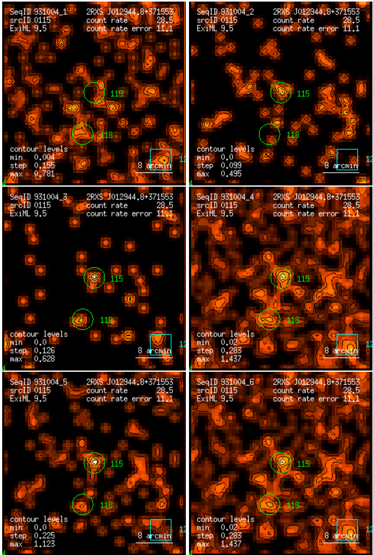
Figure 115: RASS 931004: detection 0115: band rate images, Gaussian filter: (1) PSPC channels 11 – 41, (2) 52 – 90, (3) 91 – 201, (4) 11 – 235, (5) 52 – 201, (6) 11 – 201. Broad band rates in counts/ks. Band rate contour levels in counts/ks/arcmin 2 .
