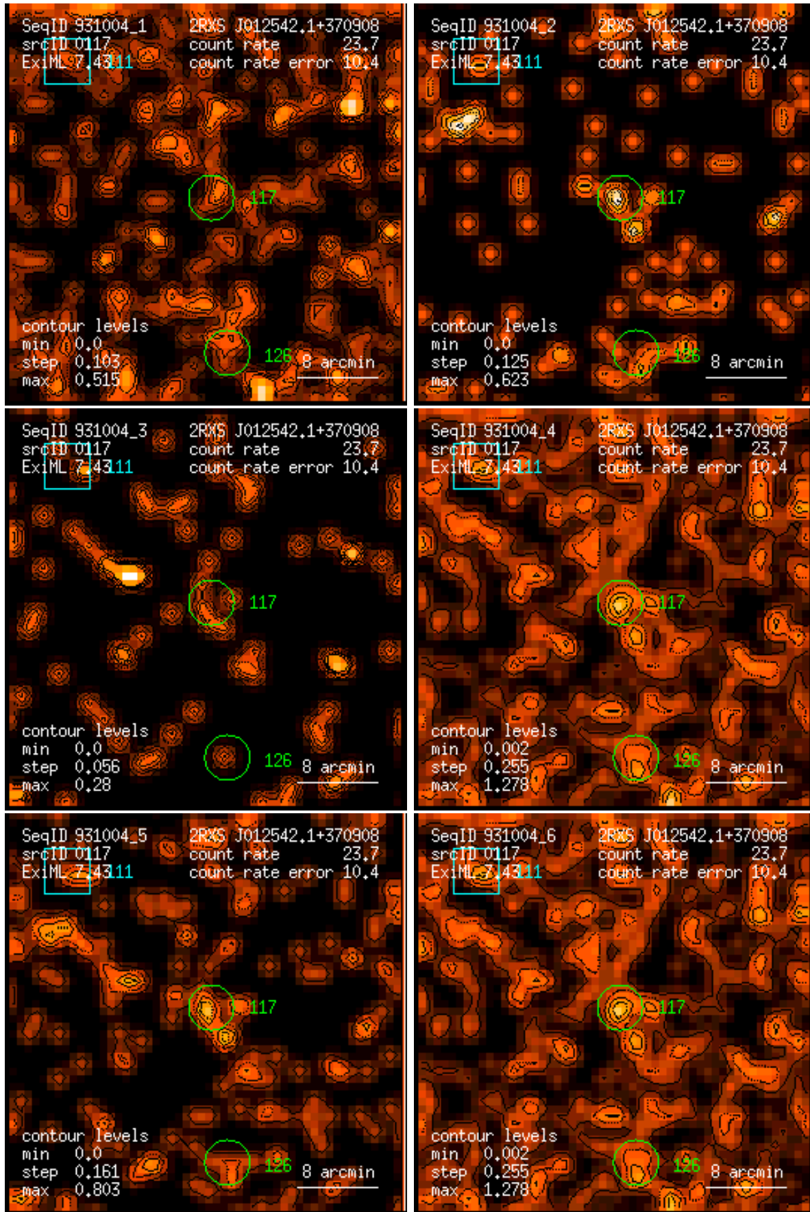
Figure 117: RASS 931004: detection 0117: band rate images, Gaussian filter: (1) PSPC channels 11 – 41, (2) 52 – 90, (3) 91 – 201, (4) 11 – 235, (5) 52 – 201, (6) 11 – 201. Broad band rates in counts/ks. Band rate contour levels in counts/ks/arcmin 2 .
