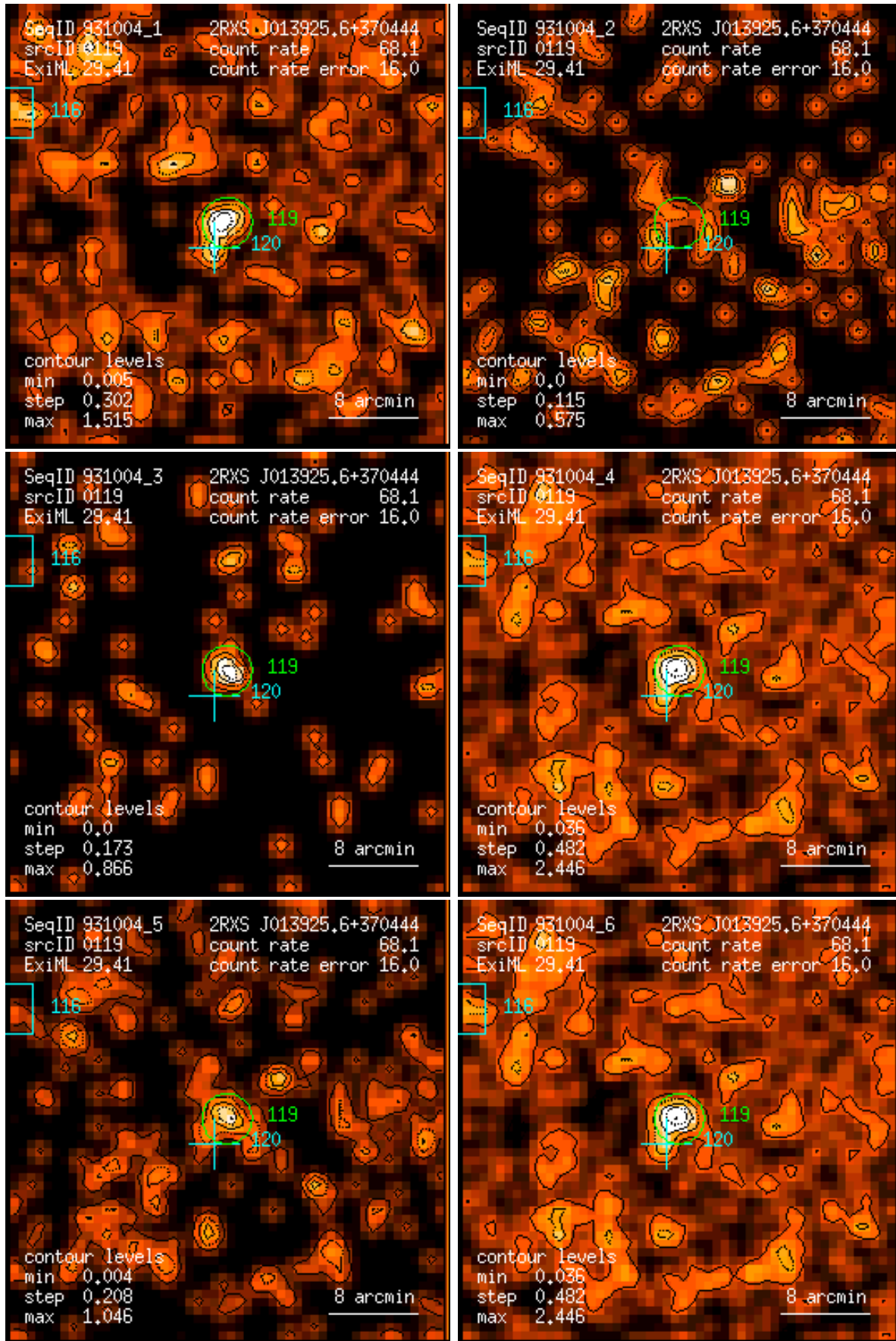
Figure 119: RASS 931004: detection 0119: band rate images, Gaussian filter: (1) PSPC channels 11 – 41, (2) 52 – 90, (3) 91 – 201, (4) 11 – 235, (5) 52 – 201, (6) 11 – 201. Broad band rates in counts/ks. Band rate contour levels in counts/ks/arcmin 2 .
