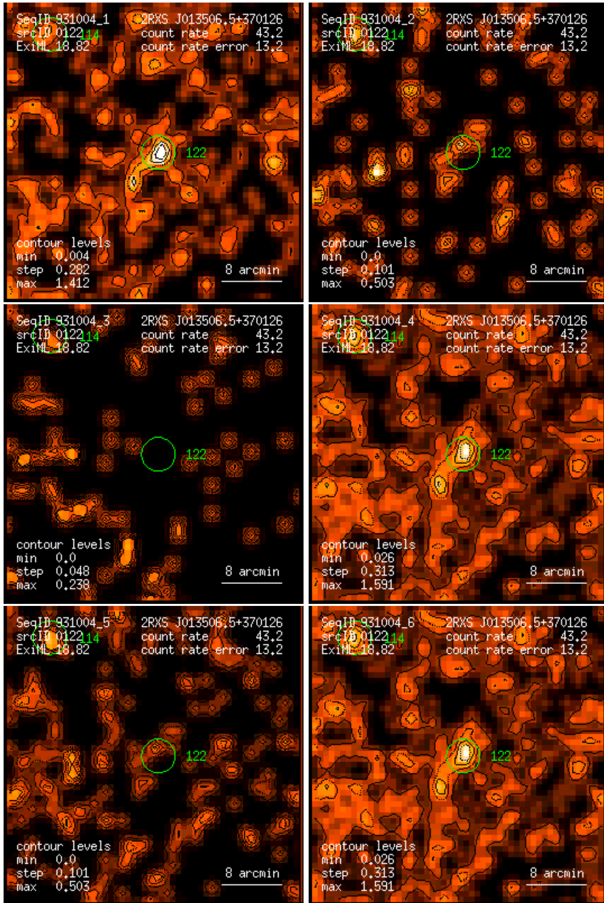
Figure 122: RASS 931004: detection 0122: band rate images, Gaussian filter: (1) PSPC channels 11 – 41, (2) 52 – 90, (3) 91 – 201, (4) 11 – 235, (5) 52 – 201, (6) 11 – 201. Broad band rates in counts/ks. Band rate contour levels in counts/ks/arcmin 2 .
