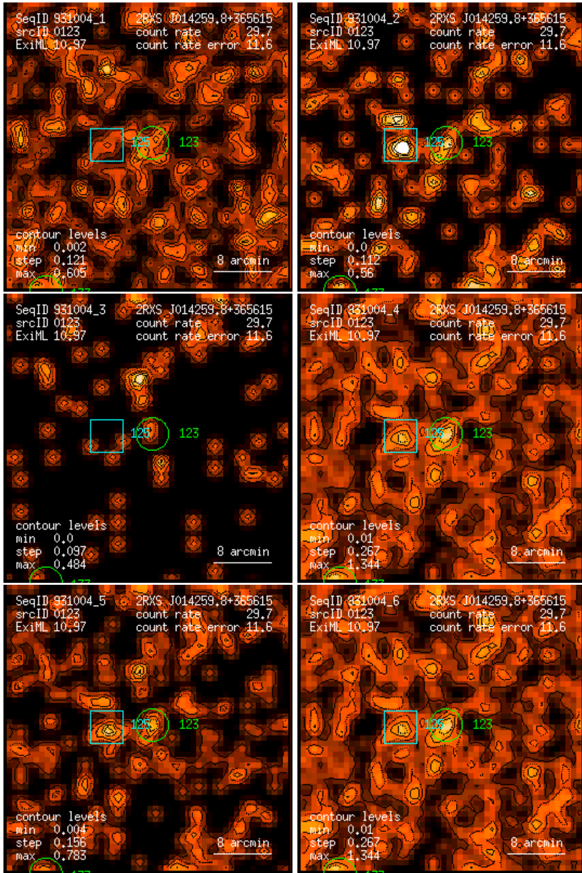
Figure 123: RASS 931004: detection 0123: band rate images, Gaussian filter: (1) PSPC channels 11 – 41, (2) 52 – 90, (3) 91 – 201, (4) 11 – 235, (5) 52 – 201, (6) 11 – 201. Broad band rates in counts/ks. Band rate contour levels in counts/ks/arcmin 2 .
