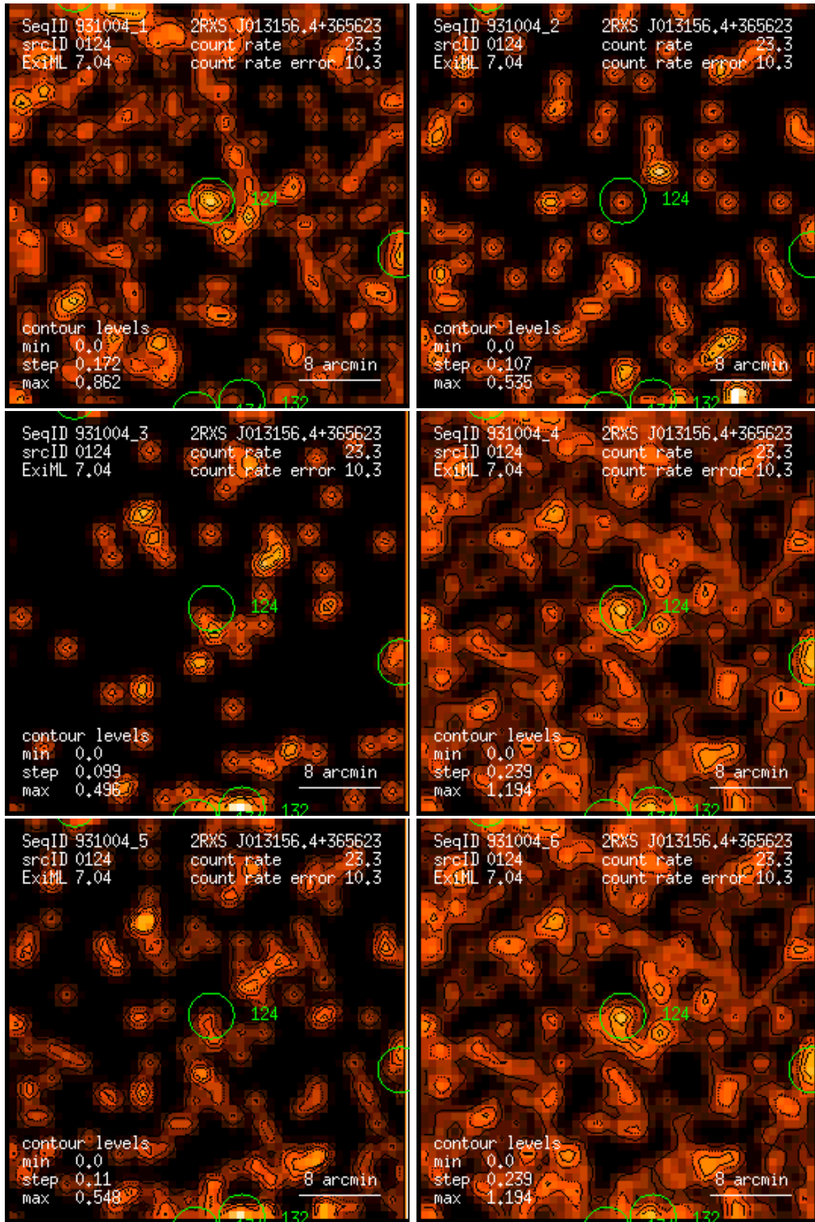
Figure 124: RASS 931004: detection 0124: band rate images, Gaussian filter: (1) PSPC channels 11 – 41, (2) 52 – 90, (3) 91 – 201, (4) 11 – 235, (5) 52 – 201, (6) 11 – 201. Broad band rates in counts/ks. Band rate contour levels in counts/ks/arcmin 2 .
