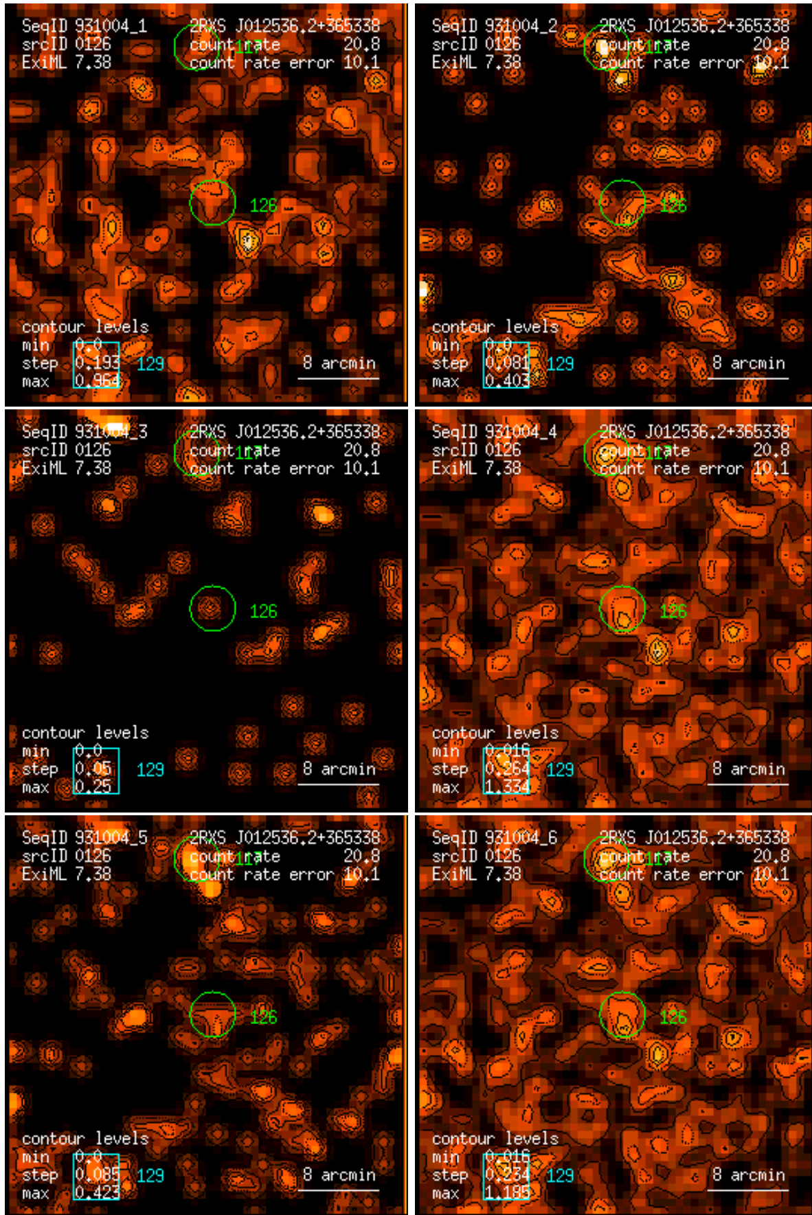
Figure 126: RASS 931004: detection 0126: band rate images, Gaussian filter: (1) PSPC channels 11 – 41, (2) 52 – 90, (3) 91 – 201, (4) 11 – 235, (5) 52 – 201, (6) 11 – 201. Broad band rates in counts/ks. Band rate contour levels in counts/ks/arcmin 2 .
