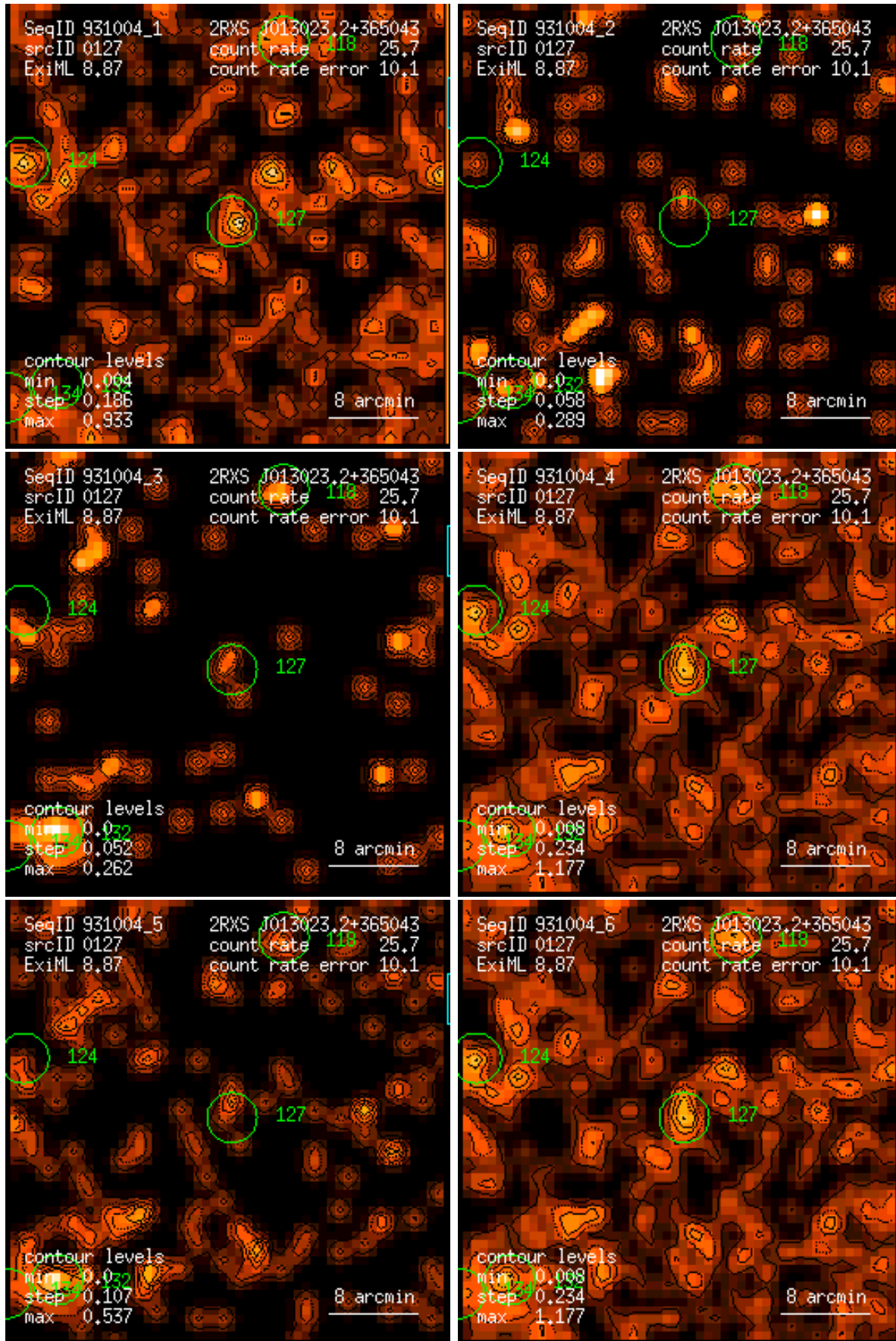
Figure 127: RASS 931004: detection 0127: band rate images, Gaussian filter: (1) PSPC channels 11 – 41, (2) 52 – 90, (3) 91 – 201, (4) 11 – 235, (5) 52 – 201, (6) 11 – 201. Broad band rates in counts/ks. Band rate contour levels in counts/ks/arcmin 2 .
