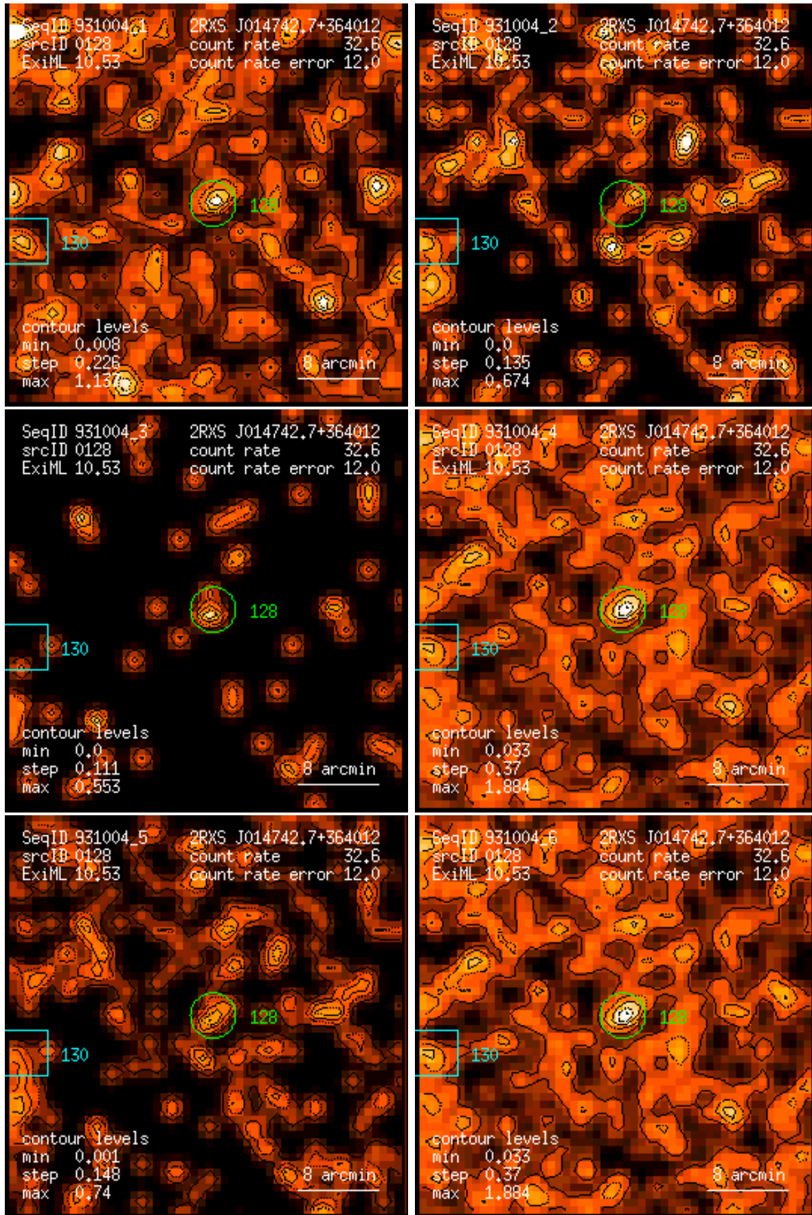
Figure 128: RASS 931004: detection 0128: band rate images, Gaussian filter: (1) PSPC channels 11 – 41, (2) 52 – 90, (3) 91 – 201, (4) 11 – 235, (5) 52 – 201, (6) 11 – 201. Broad band rates in counts/ks. Band rate contour levels in counts/ks/arcmin 2 .
