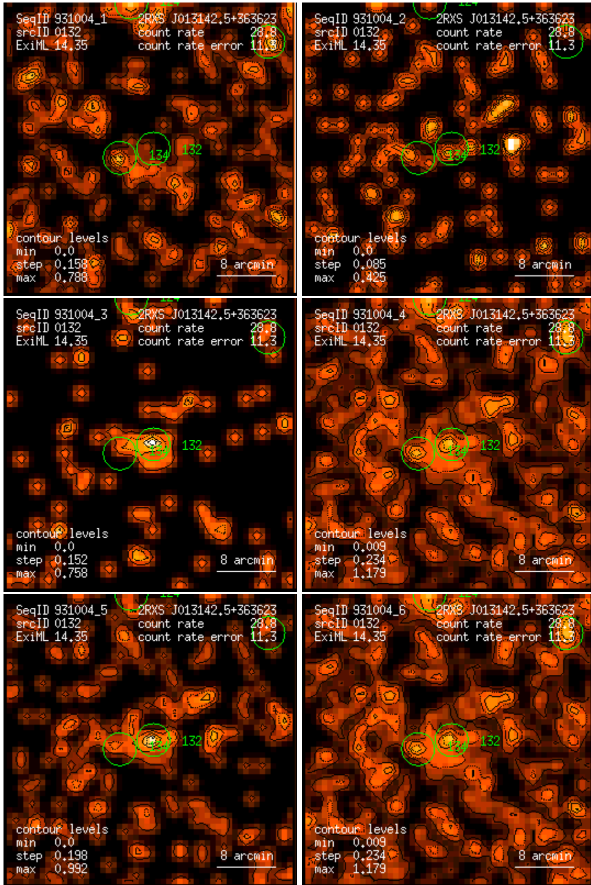
Figure 132: RASS 931004: detection 0132: band rate images, Gaussian filter: (1) PSPC channels 11 – 41, (2) 52 – 90, (3) 91 – 201, (4) 11 – 235, (5) 52 – 201, (6) 11 – 201. Broad band rates in counts/ks. Band rate contour levels in counts/ks/arcmin 2 .
