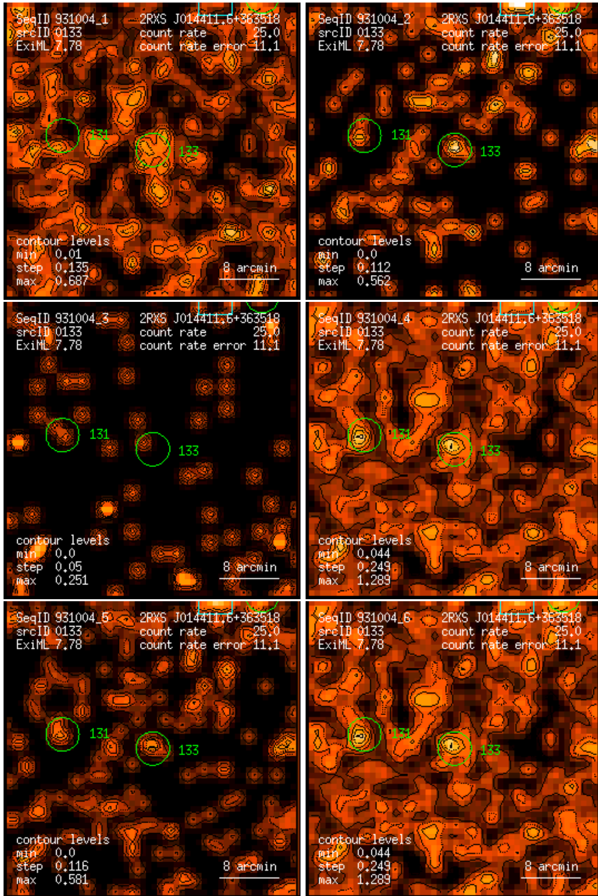
Figure 133: RASS 931004: detection 0133: band rate images, Gaussian filter: (1) PSPC channels 11 – 41, (2) 52 – 90, (3) 91 – 201, (4) 11 – 235, (5) 52 – 201, (6) 11 – 201. Broad band rates in counts/ks. Band rate contour levels in counts/ks/arcmin 2 .
