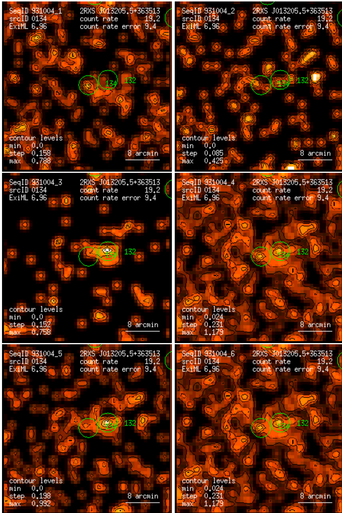
Figure 134: RASS 931004: detection 0134: band rate images, Gaussian filter: (1) PSPC channels 11 – 41, (2) 52 – 90, (3) 91 – 201, (4) 11 – 235, (5) 52 – 201, (6) 11 – 201. Broad band rates in counts/ks. Band rate contour levels in counts/ks/arcmin 2 .
