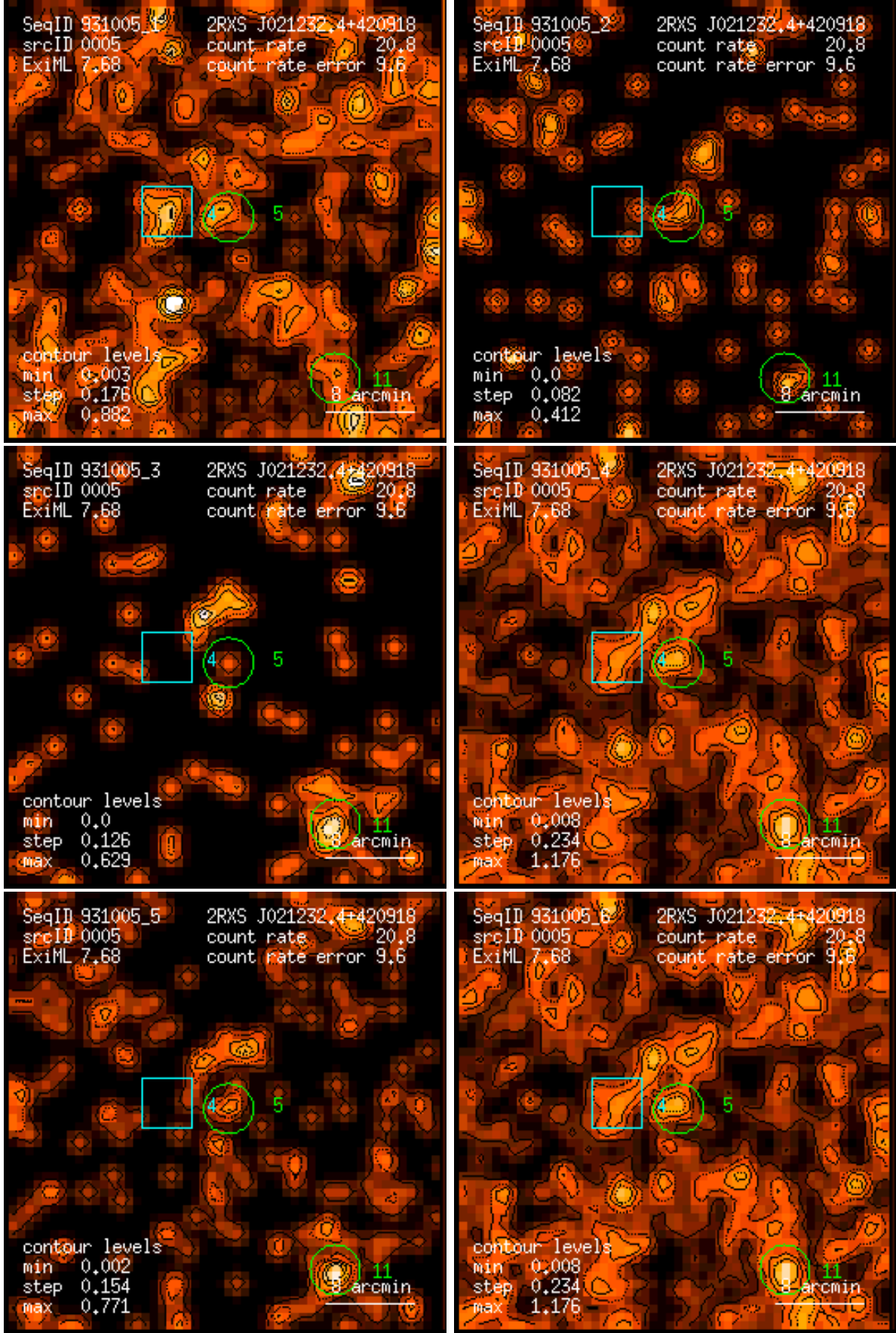
Figure 5: RASS 931005: detection 0005: band rate images, Gaussian filter: (1) PSPC channels 11 – 41, (2) 52 – 90, (3) 91 – 201, (4) 11 – 235, (5) 52 – 201, (6) 11 – 201. Broad band rates in counts/ks. Band rate contour levels in counts/ks/arcmin 2 .
