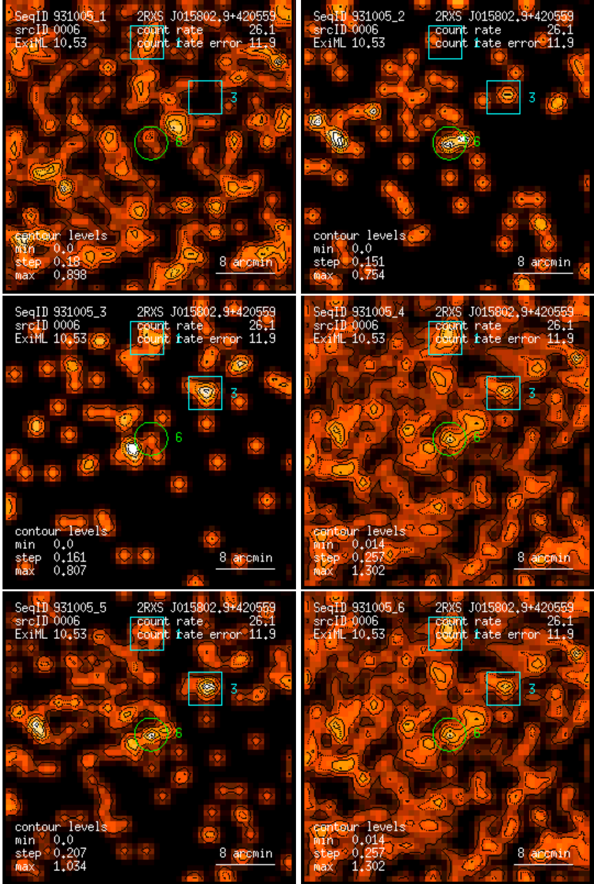
Figure 6: RASS 931005: detection 0006: band rate images, Gaussian filter: (1) PSPC channels 11 – 41, (2) 52 – 90, (3) 91 – 201, (4) 11 – 235, (5) 52 – 201, (6) 11 – 201. Broad band rates in counts/ks. Band rate contour levels in counts/ks/arcmin 2 .
