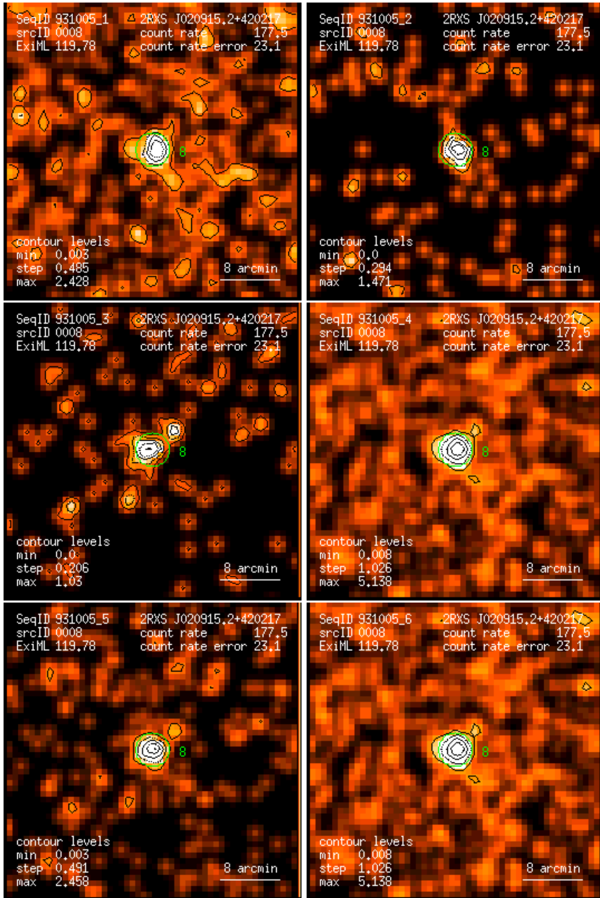
Figure 8: RASS 931005: detection 0008: band rate images, Gaussian filter: (1) PSPC channels 11 – 41, (2) 52 – 90, (3) 91 – 201, (4) 11 – 235, (5) 52 – 201, (6) 11 – 201. Broad band rates in counts/ks. Band rate contour levels in counts/ks/arcmin 2 .
