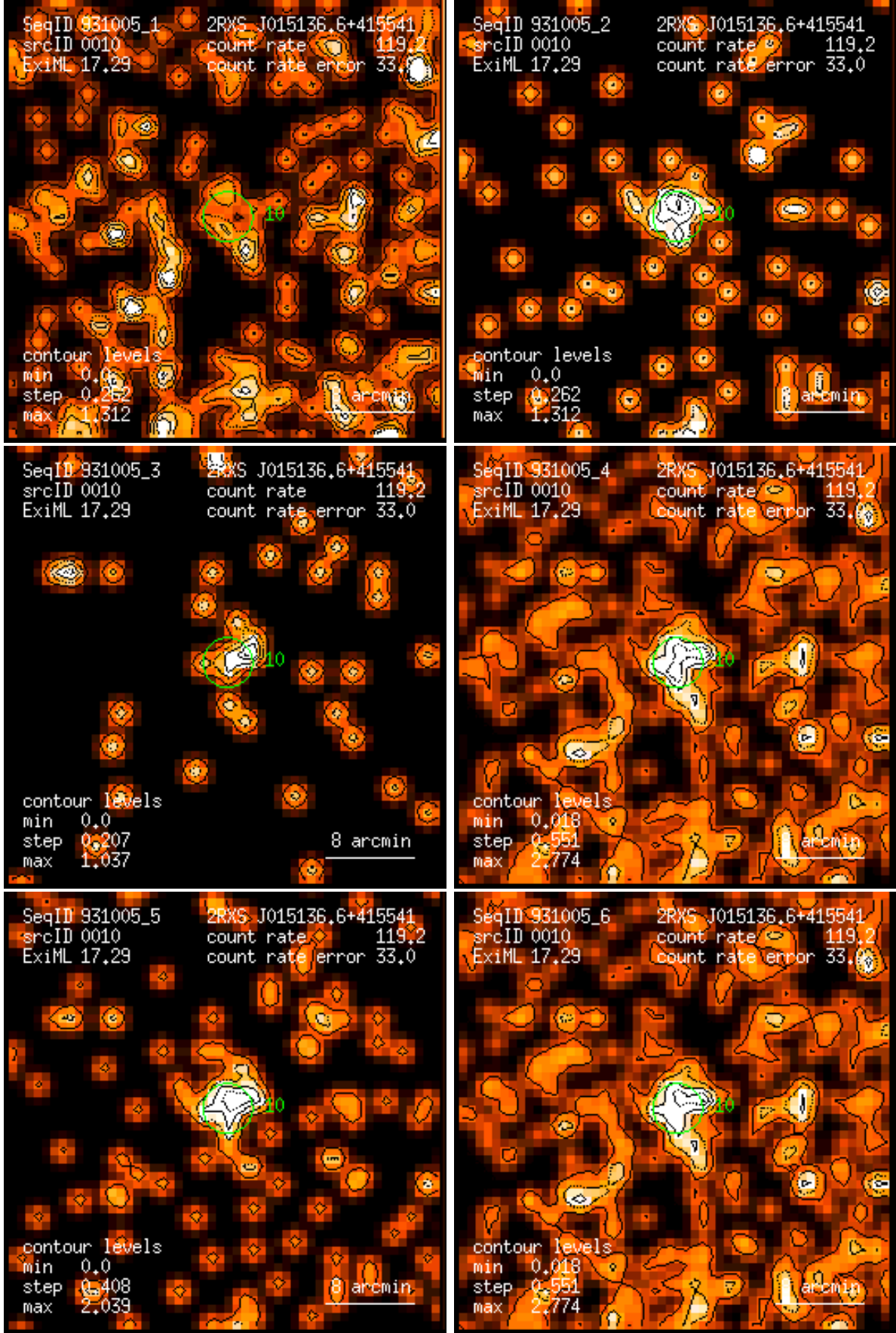
Figure 10: RASS 931005: detection 0010: band rate images, Gaussian filter: (1) PSPC channels 11 – 41, (2) 52 – 90, (3) 91 – 201, (4) 11 – 235, (5) 52 – 201, (6) 11 – 201. Broad band rates in counts/ks. Band rate contour levels in counts/ks/arcmin 2 .
