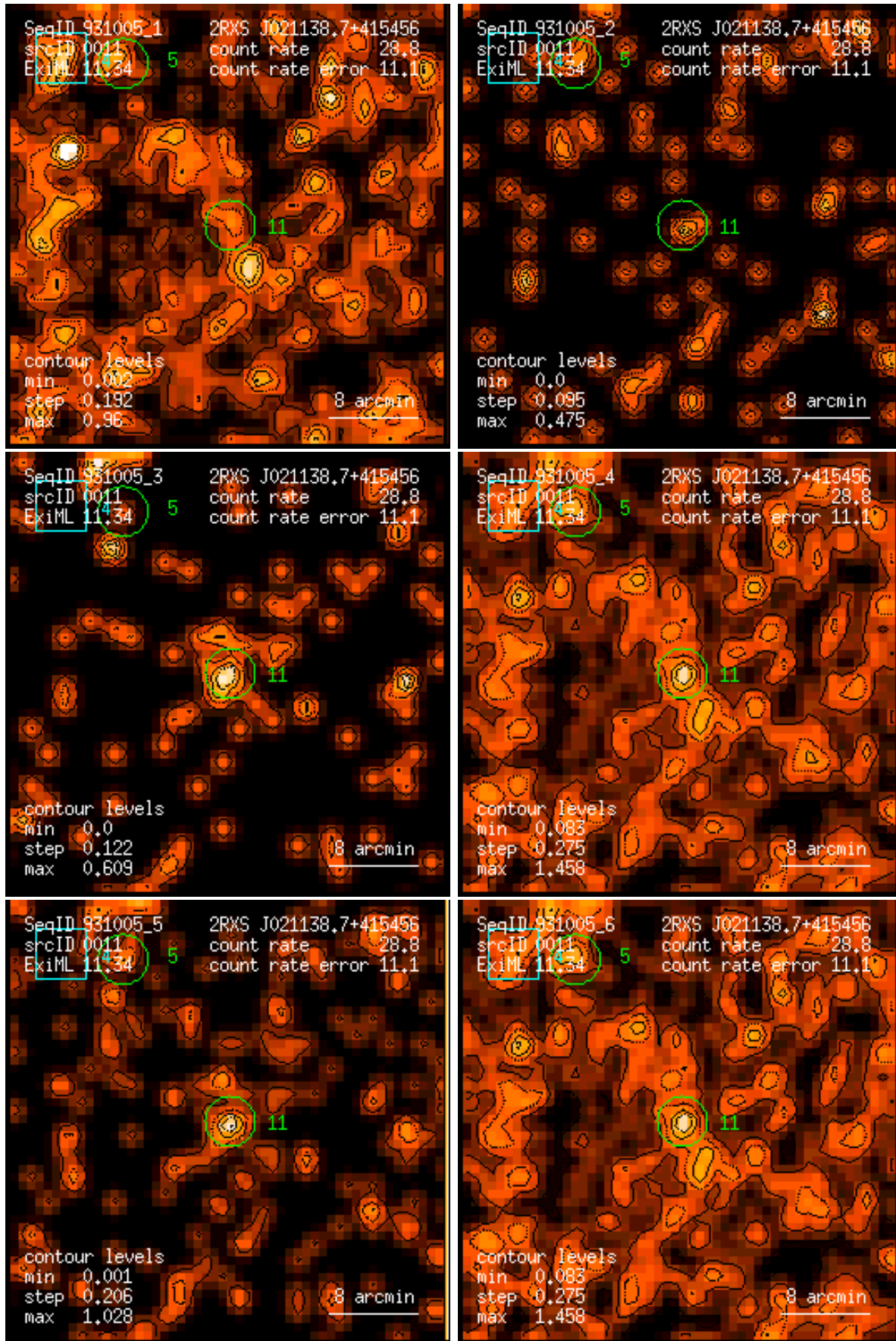
Figure 11: RASS 931005: detection 0011: band rate images, Gaussian filter: (1) PSPC channels 11 – 41, (2) 52 – 90, (3) 91 – 201, (4) 11 – 235, (5) 52 – 201, (6) 11 – 201. Broad band rates in counts/ks. Band rate contour levels in counts/ks/arcmin 2 .
