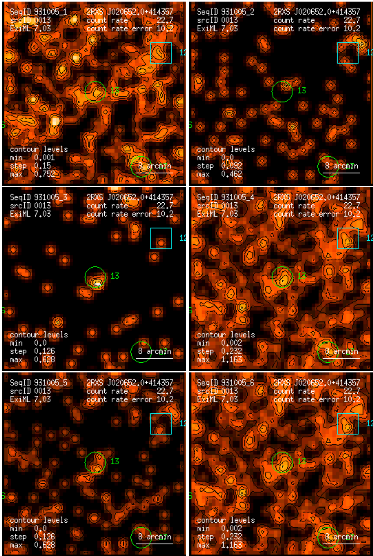
Figure 13: RASS 931005: detection 0013: band rate images, Gaussian filter: (1) PSPC channels 11 – 41, (2) 52 – 90, (3) 91 – 201, (4) 11 – 235, (5) 52 – 201, (6) 11 – 201. Broad band rates in counts/ks. Band rate contour levels in counts/ks/arcmin 2 .
