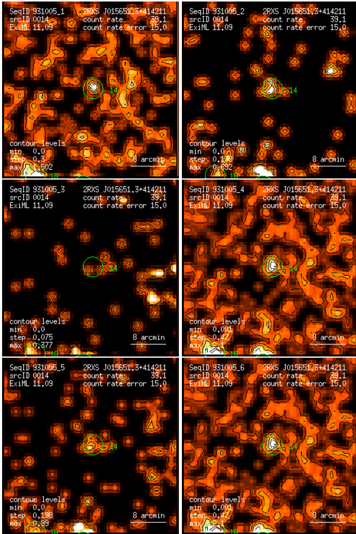
Figure 14: RASS 931005: detection 0014: band rate images, Gaussian filter: (1) PSPC channels 11 – 41, (2) 52 – 90, (3) 91 – 201, (4) 11 – 235, (5) 52 – 201, (6) 11 – 201. Broad band rates in counts/ks. Band rate contour levels in counts/ks/arcmin 2 .
