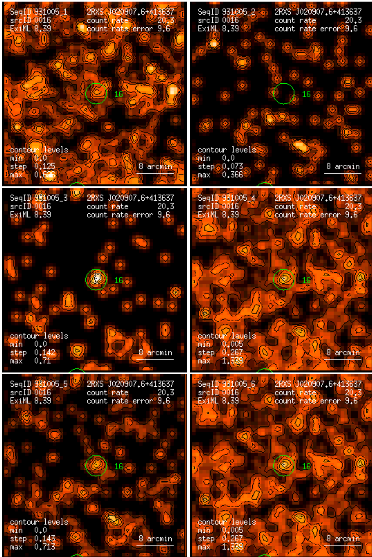
Figure 16: RASS 931005: detection 0016: band rate images, Gaussian filter: (1) PSPC channels 11 – 41, (2) 52 – 90, (3) 91 – 201, (4) 11 – 235, (5) 52 – 201, (6) 11 – 201. Broad band rates in counts/ks. Band rate contour levels in counts/ks/arcmin 2 .
