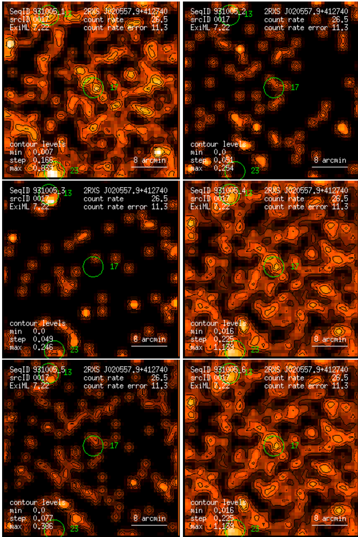
Figure 17: RASS 931005: detection 0017: band rate images, Gaussian filter: (1) PSPC channels 11 – 41, (2) 52 – 90, (3) 91 – 201, (4) 11 – 235, (5) 52 – 201, (6) 11 – 201. Broad band rates in counts/ks. Band rate contour levels in counts/ks/arcmin 2 .
