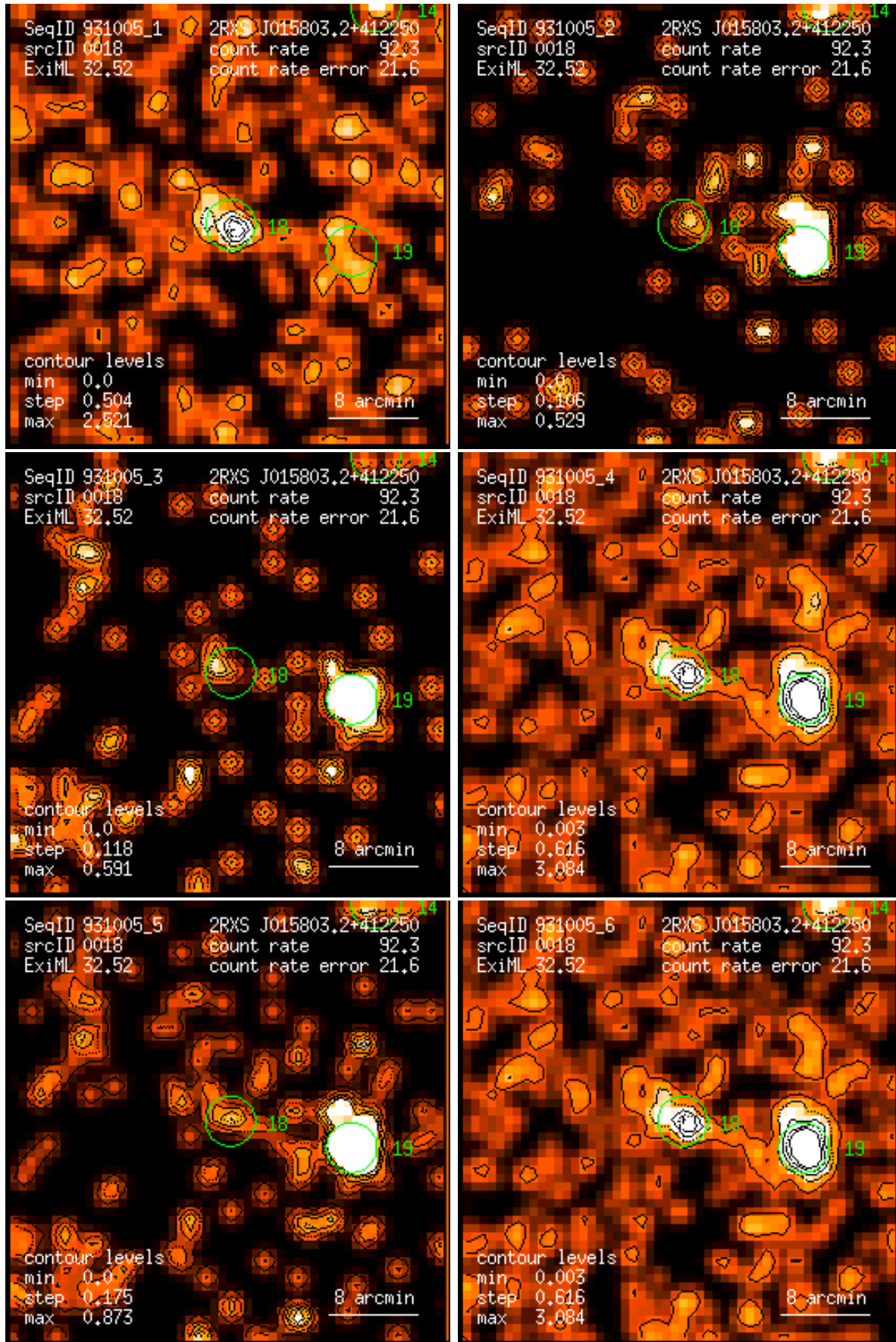
Figure 18: RASS 931005: detection 0018: band rate images, Gaussian filter: (1) PSPC channels 11 – 41, (2) 52 – 90, (3) 91 – 201, (4) 11 – 235, (5) 52 – 201, (6) 11 – 201. Broad band rates in counts/ks. Band rate contour levels in counts/ks/arcmin 2 .
