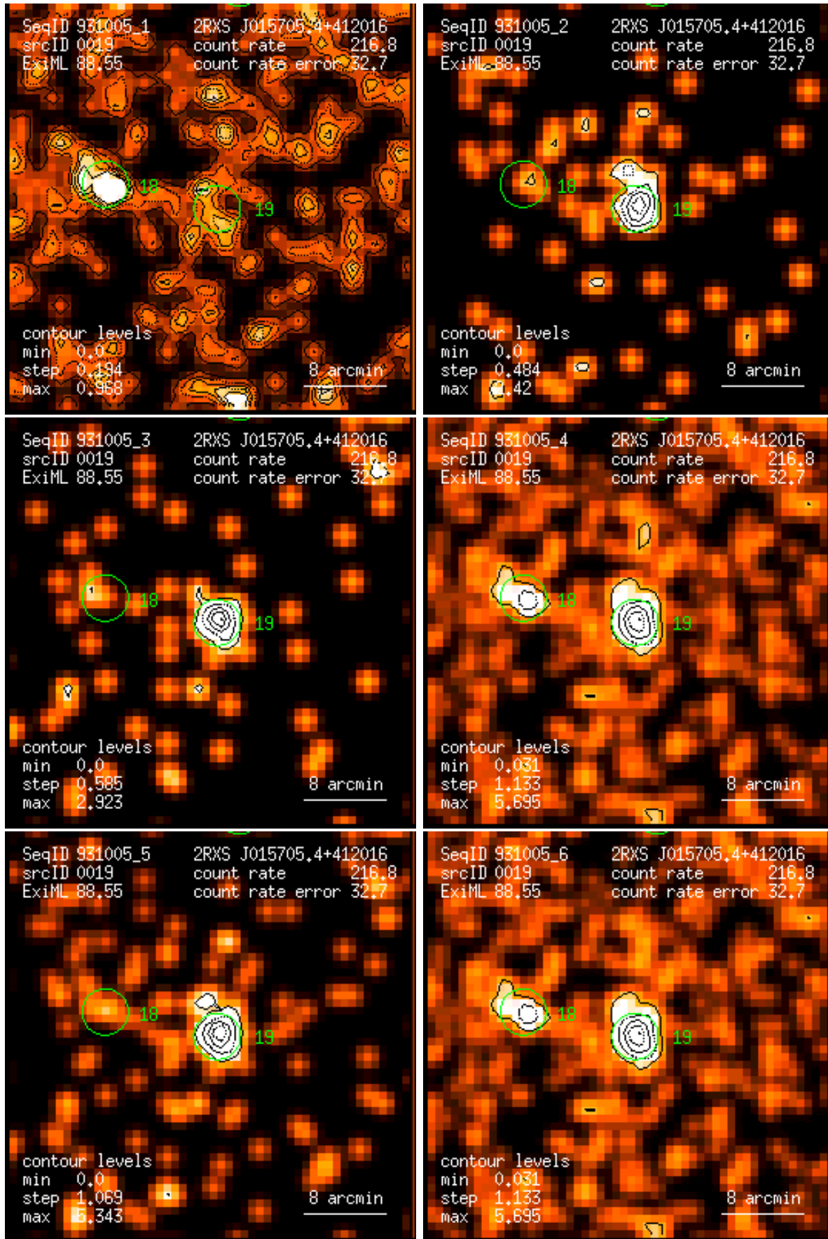
Figure 19: RASS 931005: detection 0019: band rate images, Gaussian filter: (1) PSPC channels 11 – 41, (2) 52 – 90, (3) 91 – 201, (4) 11 – 235, (5) 52 – 201, (6) 11 – 201. Broad band rates in counts/ks. Band rate contour levels in counts/ks/arcmin 2 .
