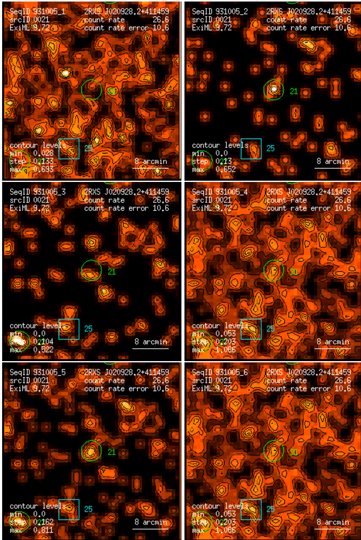
Figure 21: RASS 931005: detection 0021: band rate images, Gaussian filter: (1) PSPC channels 11 – 41, (2) 52 – 90, (3) 91 – 201, (4) 11 – 235, (5) 52 – 201, (6) 11 – 201. Broad band rates in counts/ks. Band rate contour levels in counts/ks/arcmin 2 .
