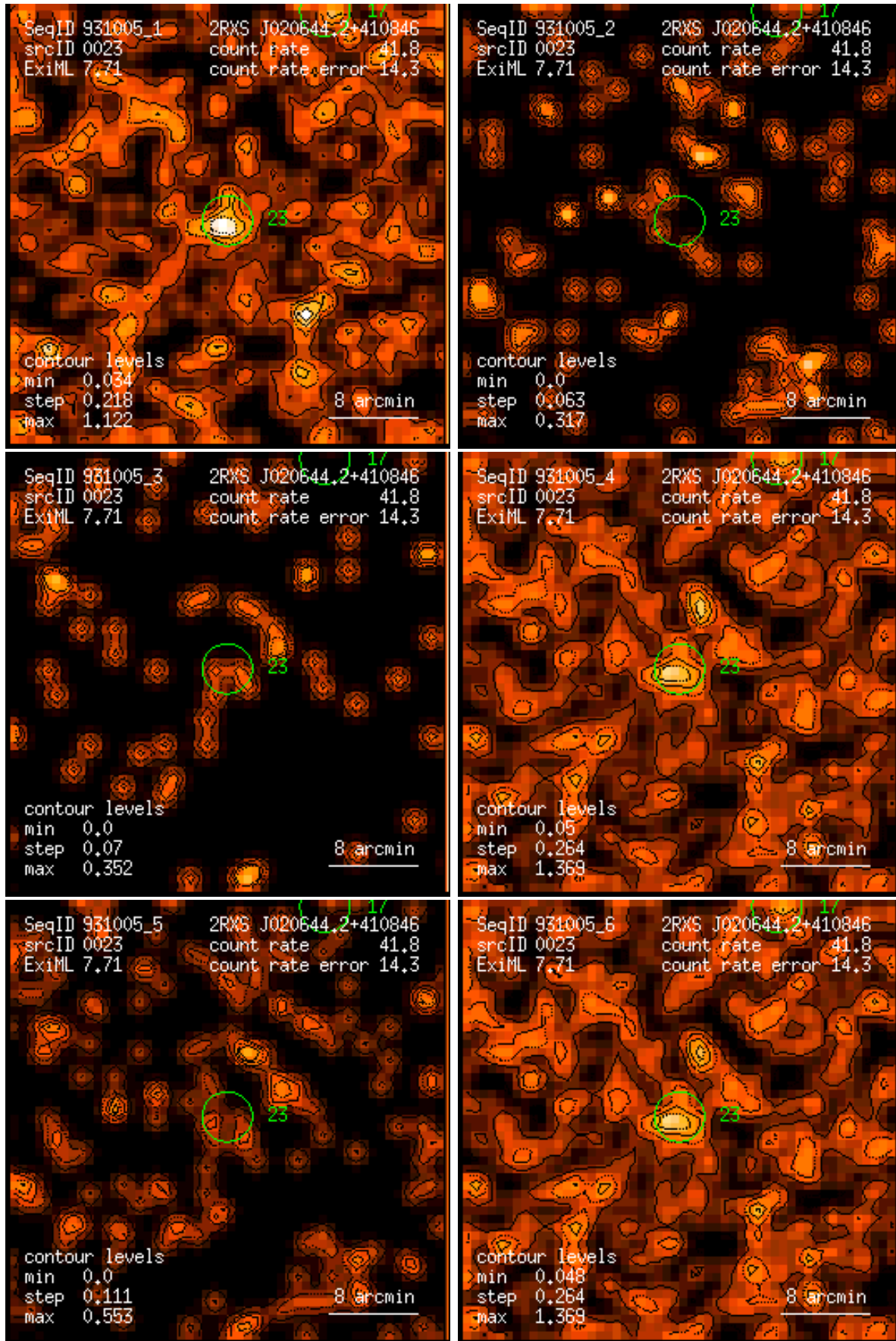
Figure 23: RASS 931005: detection 0023: band rate images, Gaussian filter: (1) PSPC channels 11 – 41, (2) 52 – 90, (3) 91 – 201, (4) 11 – 235, (5) 52 – 201, (6) 11 – 201. Broad band rates in counts/ks. Band rate contour levels in counts/ks/arcmin 2 .
