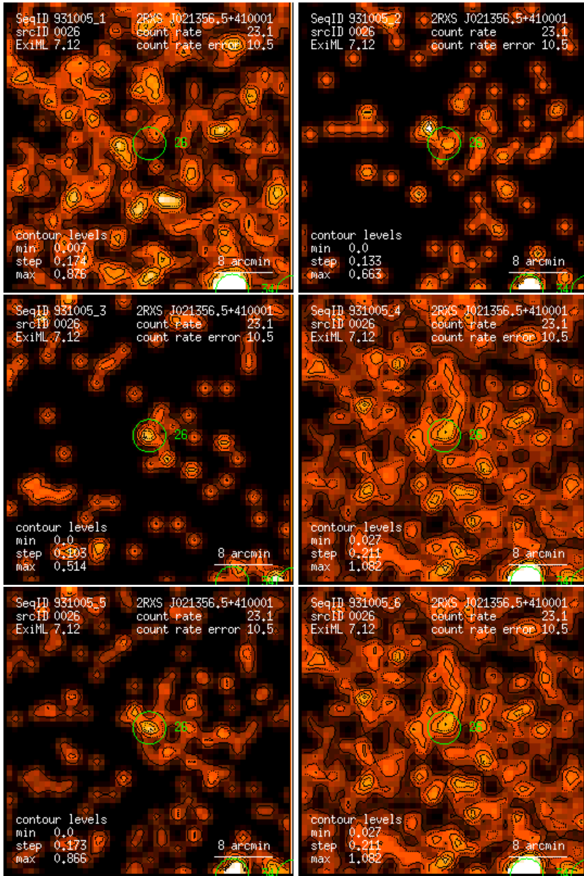
Figure 26: RASS 931005: detection 0026: band rate images, Gaussian filter: (1) PSPC channels 11 – 41, (2) 52 – 90, (3) 91 – 201, (4) 11 – 235, (5) 52 – 201, (6) 11 – 201. Broad band rates in counts/ks. Band rate contour levels in counts/ks/arcmin 2 .
