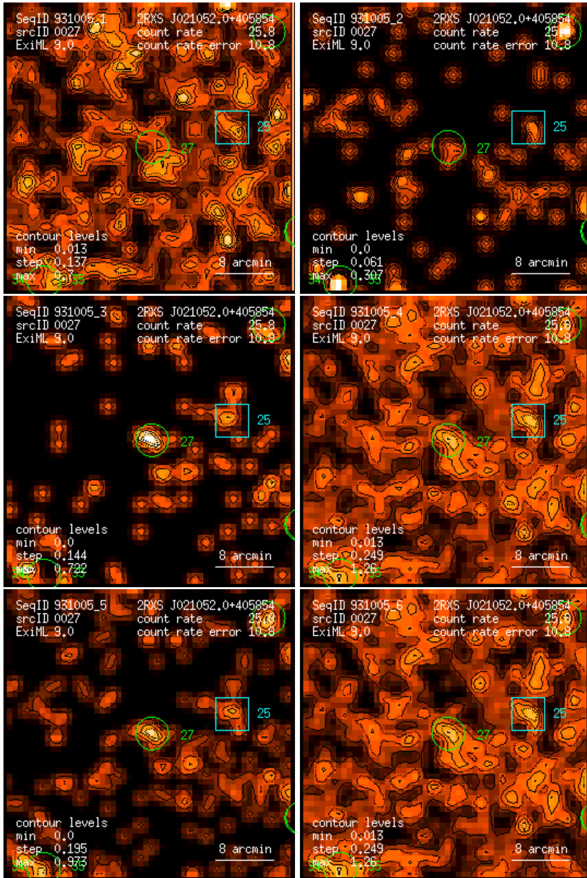
Figure 27: RASS 931005: detection 0027: band rate images, Gaussian filter: (1) PSPC channels 11 – 41, (2) 52 – 90, (3) 91 – 201, (4) 11 – 235, (5) 52 – 201, (6) 11 – 201. Broad band rates in counts/ks. Band rate contour levels in counts/ks/arcmin 2 .
