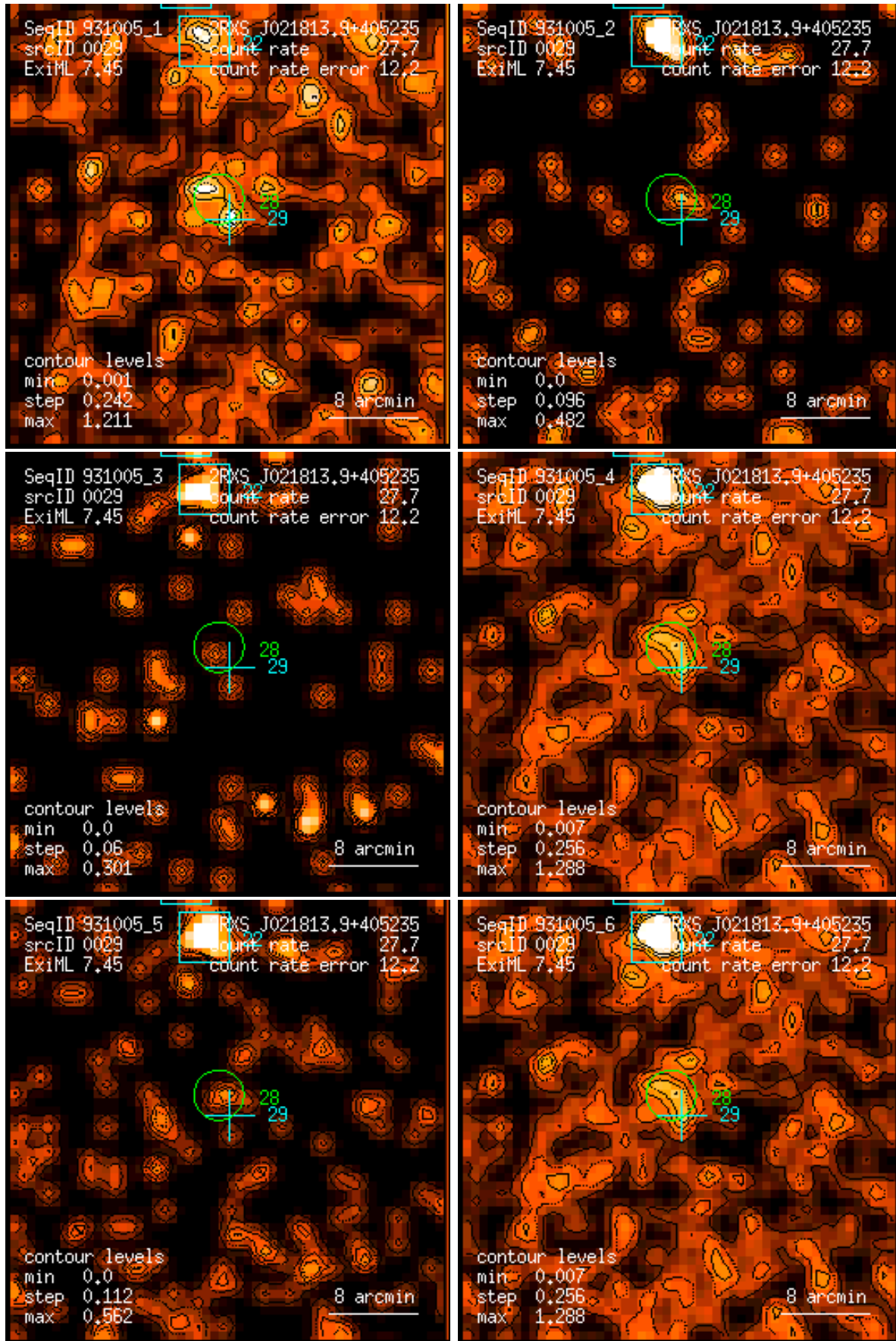
Figure 29: RASS 931005: detection 0029: band rate images, Gaussian filter: (1) PSPC channels 11 – 41, (2) 52 – 90, (3) 91 – 201, (4) 11 – 235, (5) 52 – 201, (6) 11 – 201. Broad band rates in counts/ks. Band rate contour levels in counts/ks/arcmin 2 .
