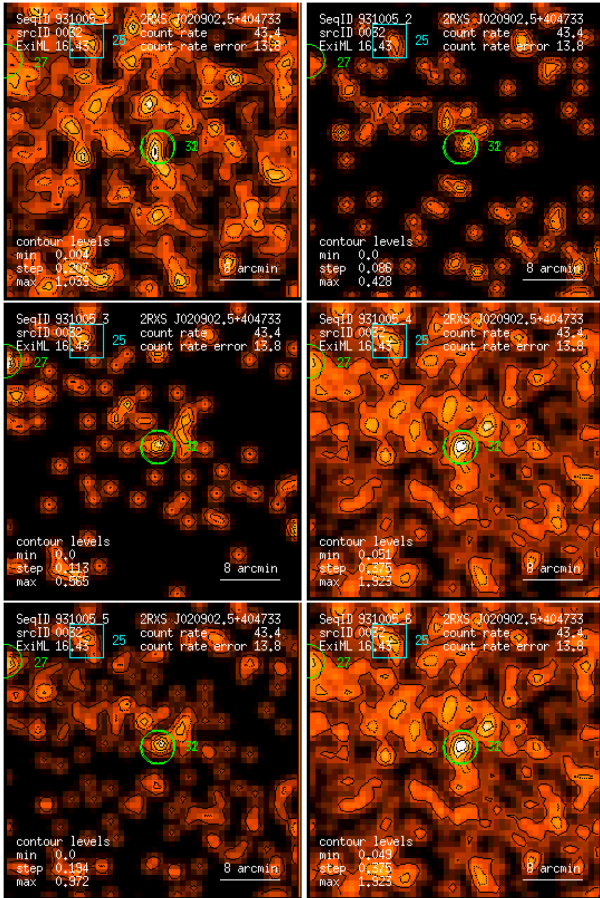
Figure 32: RASS 931005: detection 0032: band rate images, Gaussian filter: (1) PSPC channels 11 – 41, (2) 52 – 90, (3) 91 – 201, (4) 11 – 235, (5) 52 – 201, (6) 11 – 201. Broad band rates in counts/ks. Band rate contour levels in counts/ks/arcmin 2 .
