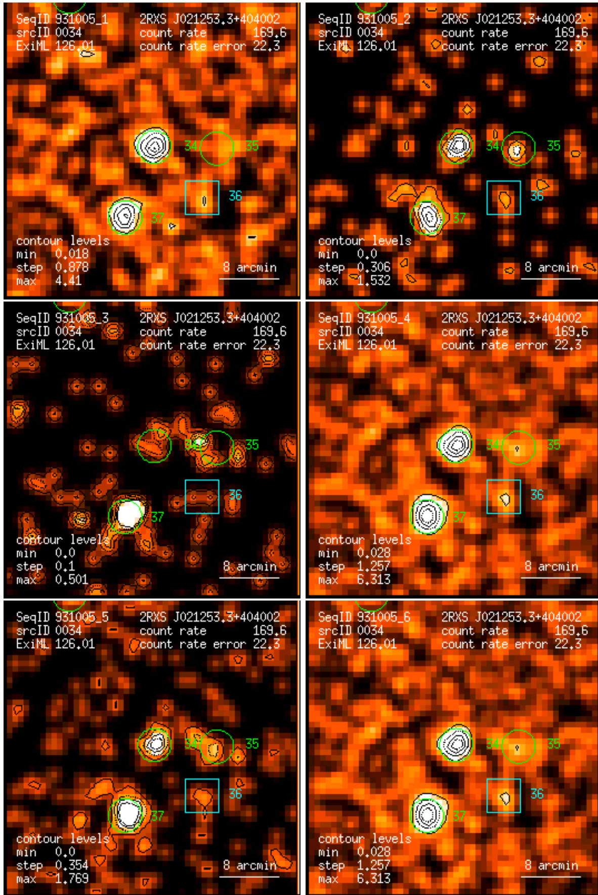
Figure 34: RASS 931005: detection 0034: band rate images, Gaussian filter: (1) PSPC channels 11 – 41, (2) 52 – 90, (3) 91 – 201, (4) 11 – 235, (5) 52 – 201, (6) 11 – 201. Broad band rates in counts/ks. Band rate contour levels in counts/ks/arcmin 2 .
