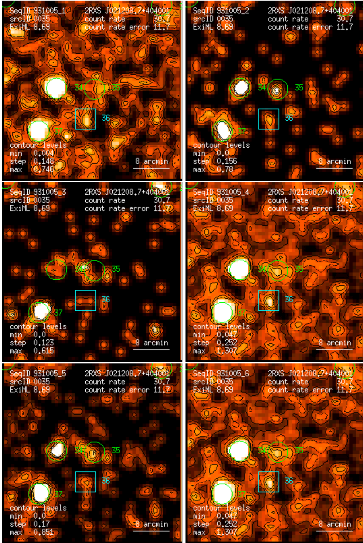
Figure 35: RASS 931005: detection 0035: band rate images, Gaussian filter: (1) PSPC channels 11 – 41, (2) 52 – 90, (3) 91 – 201, (4) 11 – 235, (5) 52 – 201, (6) 11 – 201. Broad band rates in counts/ks. Band rate contour levels in counts/ks/arcmin 2 .
