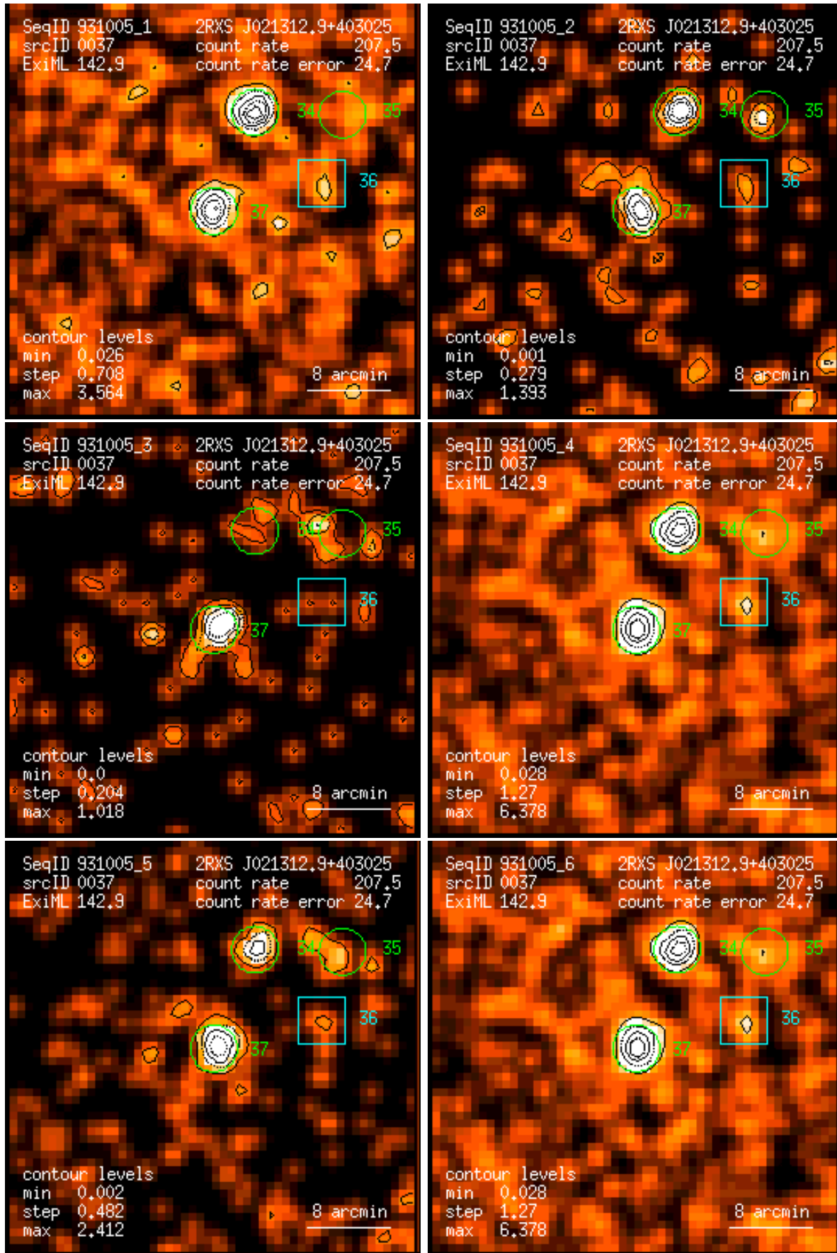
Figure 37: RASS 931005: detection 0037: band rate images, Gaussian filter: (1) PSPC channels 11 – 41, (2) 52 – 90, (3) 91 – 201, (4) 11 – 235, (5) 52 – 201, (6) 11 – 201. Broad band rates in counts/ks. Band rate contour levels in counts/ks/arcmin 2 .
