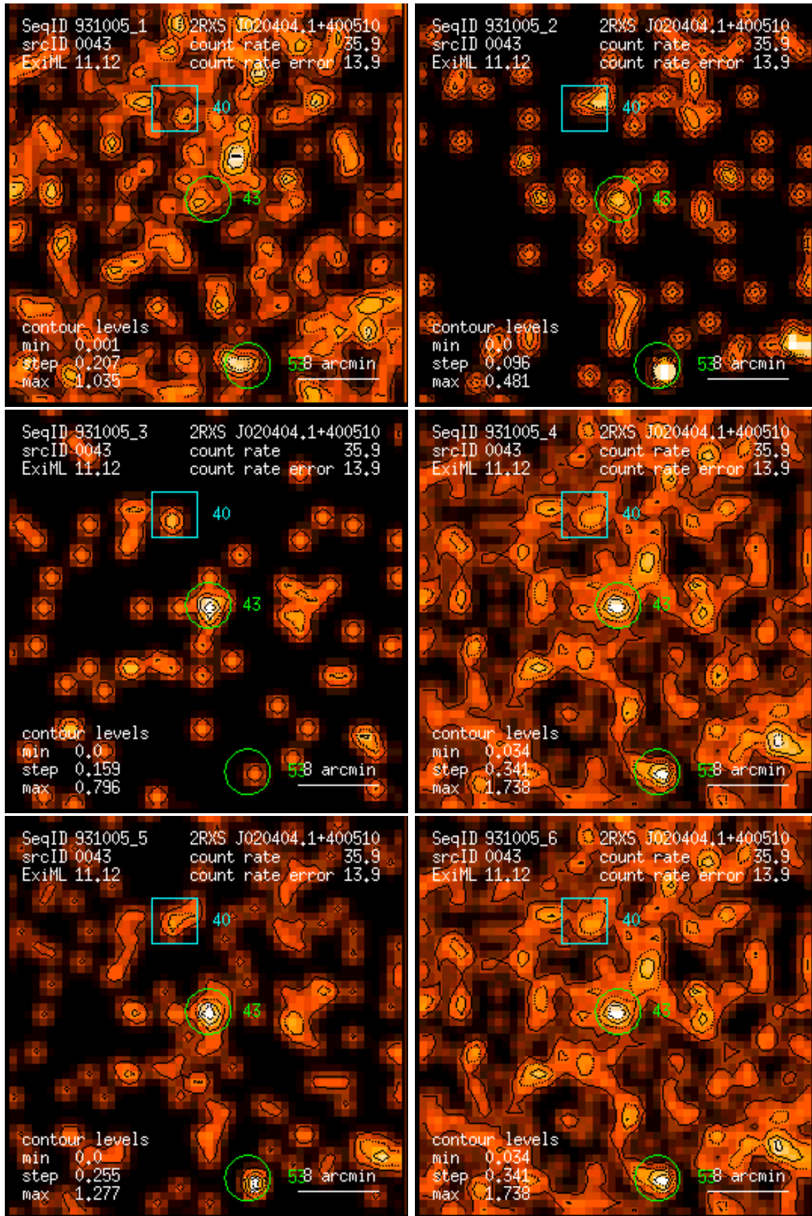
Figure 43: RASS 931005: detection 0043: band rate images, Gaussian filter: (1) PSPC channels 11 – 41, (2) 52 – 90, (3) 91 – 201, (4) 11 – 235, (5) 52 – 201, (6) 11 – 201. Broad band rates in counts/ks. Band rate contour levels in counts/ks/arcmin 2 .
