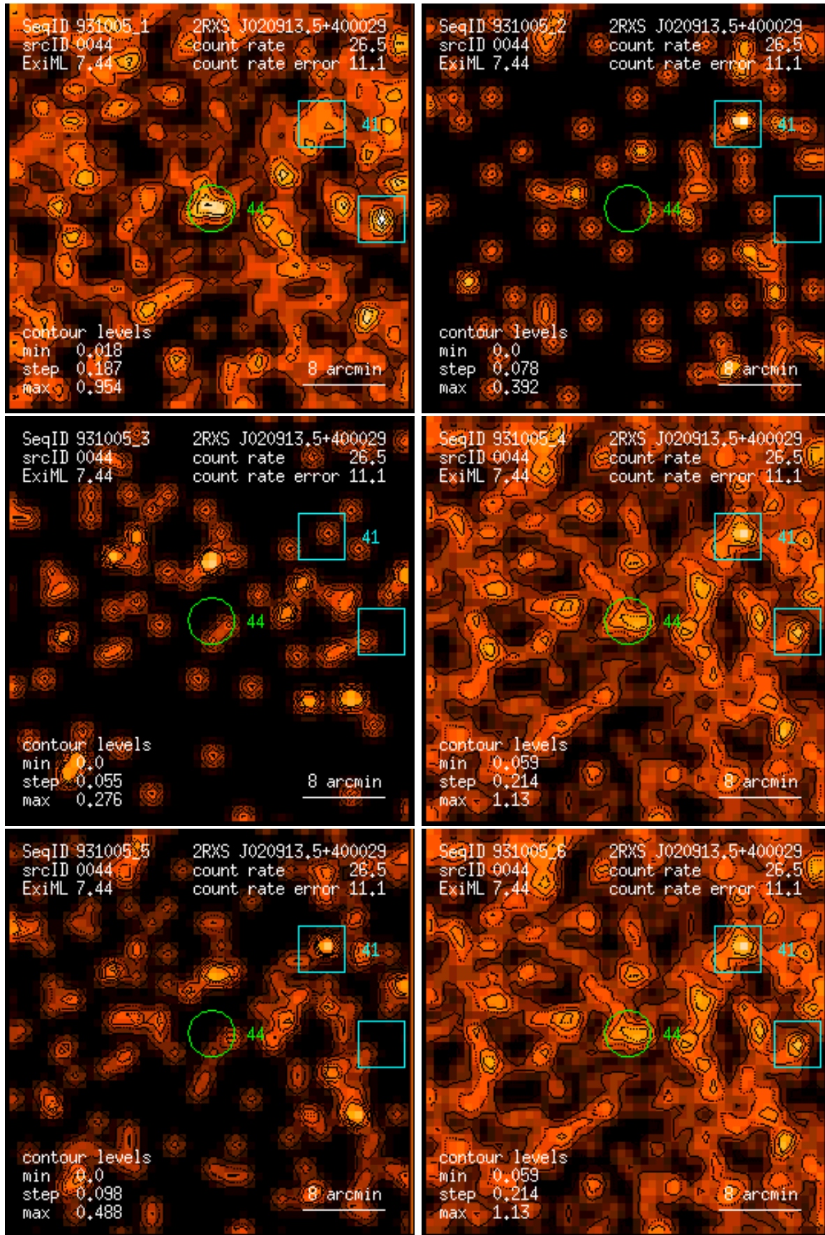
Figure 44: RASS 931005: detection 0044: band rate images, Gaussian filter: (1) PSPC channels 11 – 41, (2) 52 – 90, (3) 91 – 201, (4) 11 – 235, (5) 52 – 201, (6) 11 – 201. Broad band rates in counts/ks. Band rate contour levels in counts/ks/arcmin 2 .
