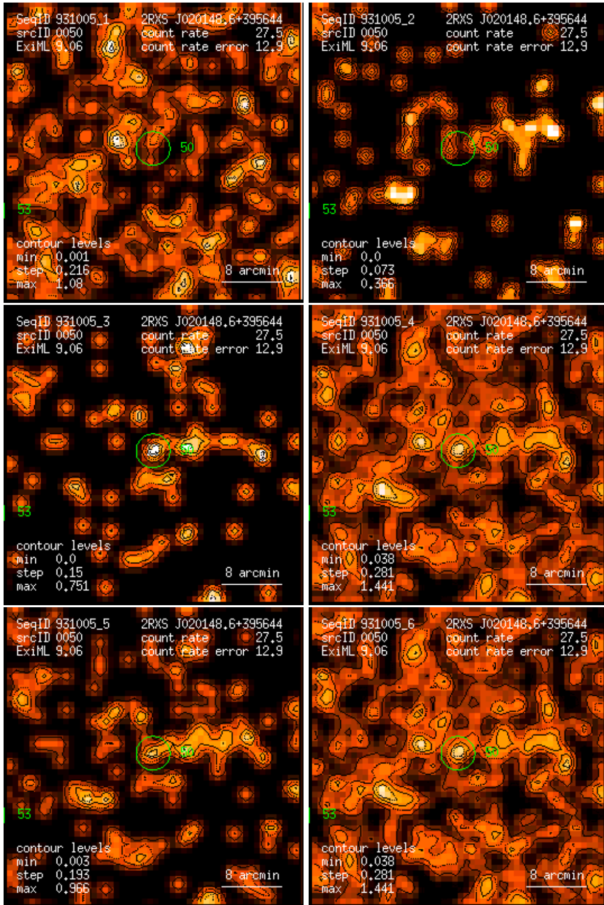
Figure 50: RASS 931005: detection 0050: band rate images, Gaussian filter: (1) PSPC channels 11 – 41, (2) 52 – 90, (3) 91 – 201, (4) 11 – 235, (5) 52 – 201, (6) 11 – 201. Broad band rates in counts/ks. Band rate contour levels in counts/ks/arcmin 2 .
