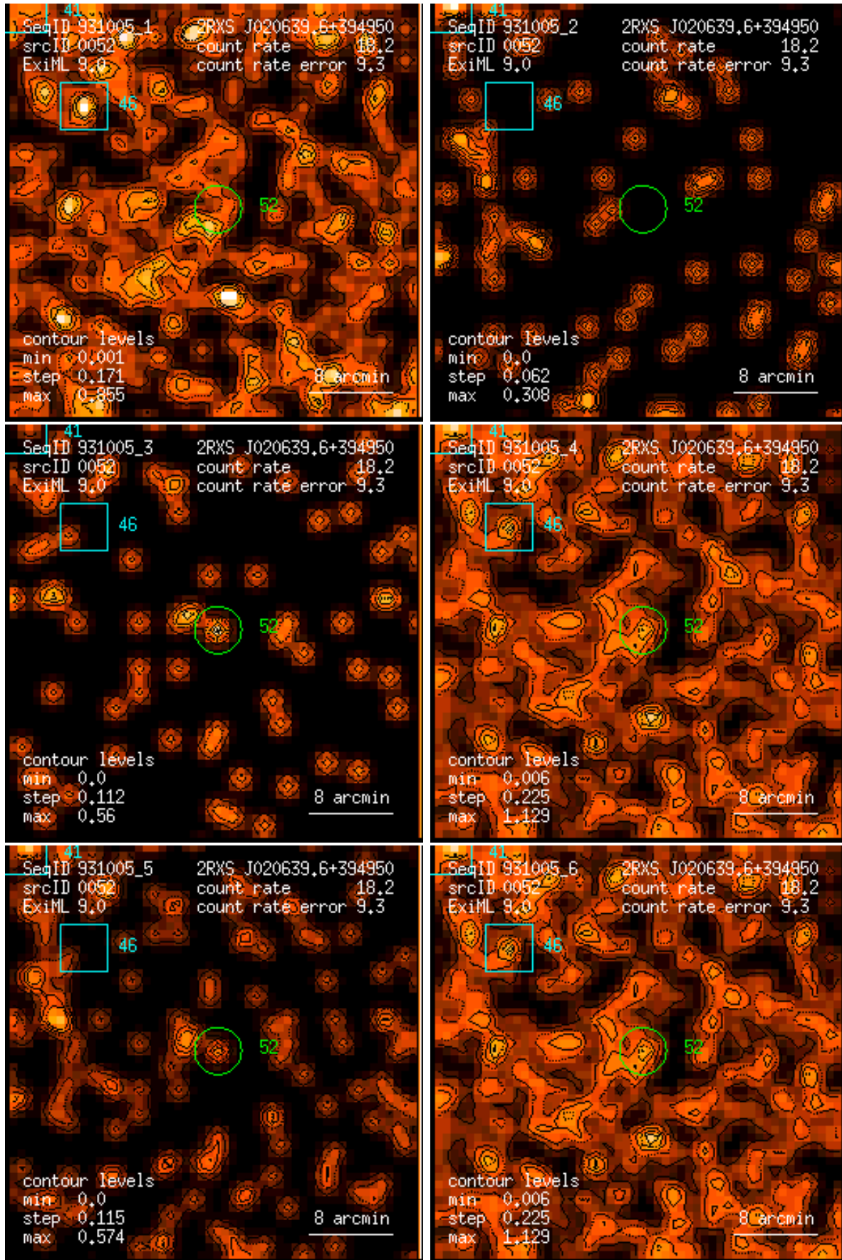
Figure 52: RASS 931005: detection 0052: band rate images, Gaussian filter: (1) PSPC channels 11 – 41, (2) 52 – 90, (3) 91 – 201, (4) 11 – 235, (5) 52 – 201, (6) 11 – 201. Broad band rates in counts/ks. Band rate contour levels in counts/ks/arcmin 2 .
