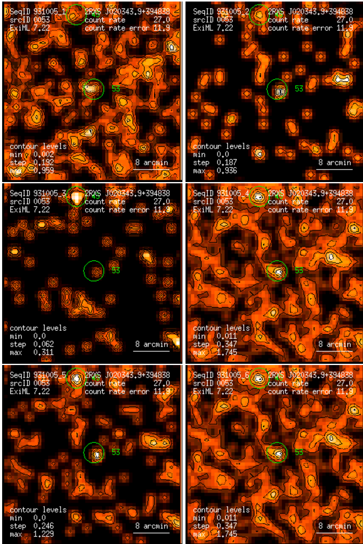
Figure 53: RASS 931005: detection 0053: band rate images, Gaussian filter: (1) PSPC channels 11 – 41, (2) 52 – 90, (3) 91 – 201, (4) 11 – 235, (5) 52 – 201, (6) 11 – 201. Broad band rates in counts/ks. Band rate contour levels in counts/ks/arcmin 2 .
