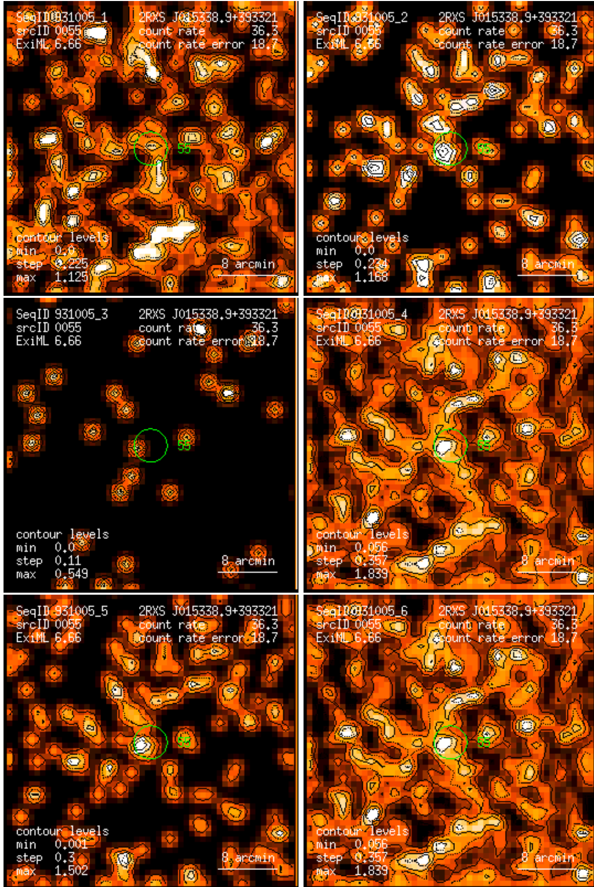
Figure 55: RASS 931005: detection 0055: band rate images, Gaussian filter: (1) PSPC channels 11 – 41, (2) 52 – 90, (3) 91 – 201, (4) 11 – 235, (5) 52 – 201, (6) 11 – 201. Broad band rates in counts/ks. Band rate contour levels in counts/ks/arcmin 2 .
