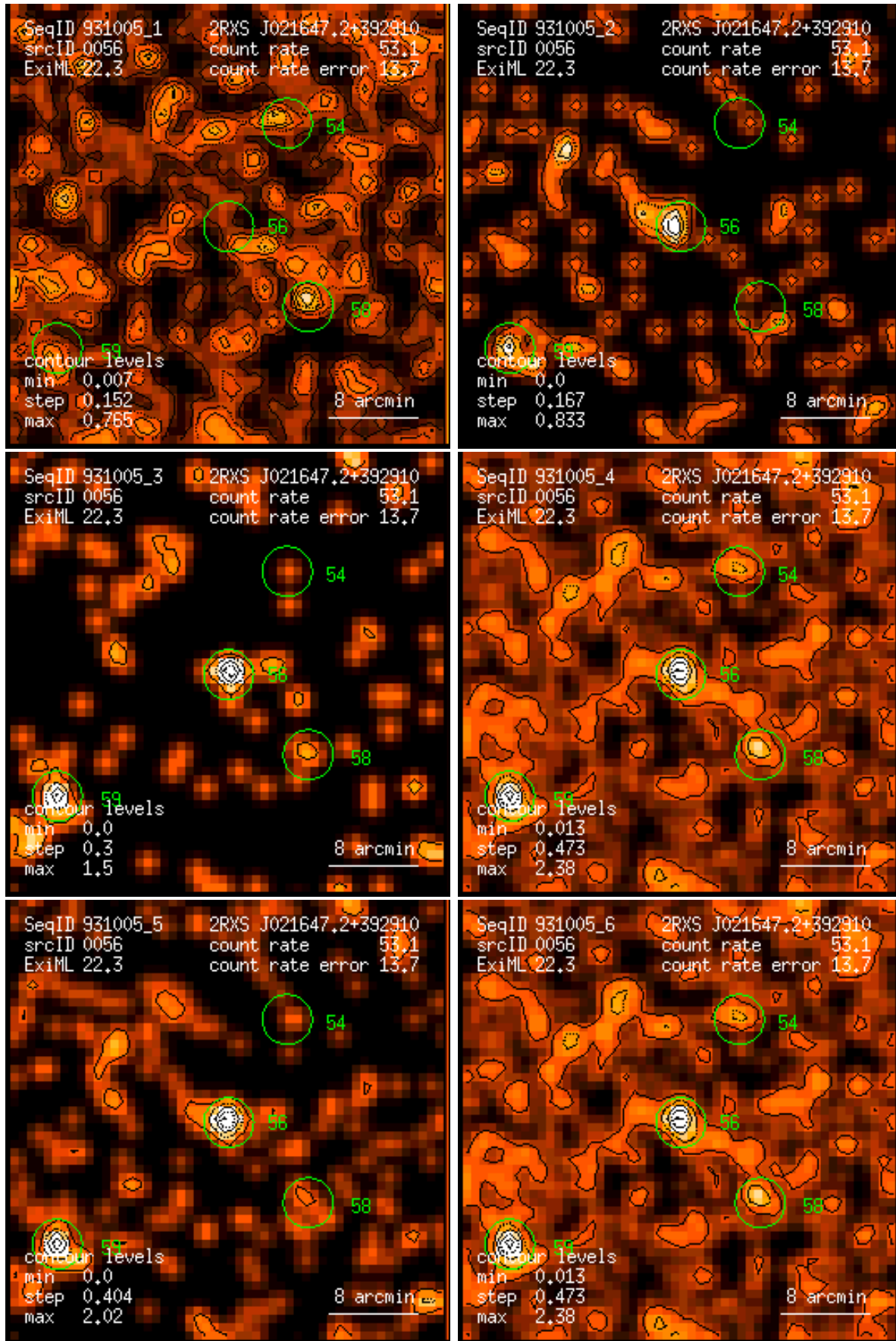
Figure 56: RASS 931005: detection 0056: band rate images, Gaussian filter: (1) PSPC channels 11 – 41, (2) 52 – 90, (3) 91 – 201, (4) 11 – 235, (5) 52 – 201, (6) 11 – 201. Broad band rates in counts/ks. Band rate contour levels in counts/ks/arcmin 2 .
