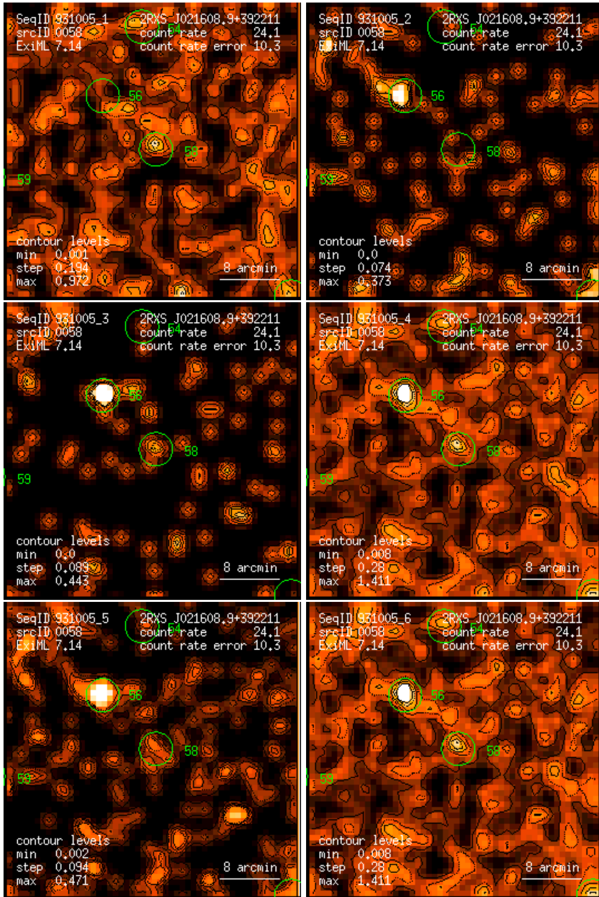
Figure 58: RASS 931005: detection 0058: band rate images, Gaussian filter: (1) PSPC channels 11 – 41, (2) 52 – 90, (3) 91 – 201, (4) 11 – 235, (5) 52 – 201, (6) 11 – 201. Broad band rates in counts/ks. Band rate contour levels in counts/ks/arcmin 2 .
