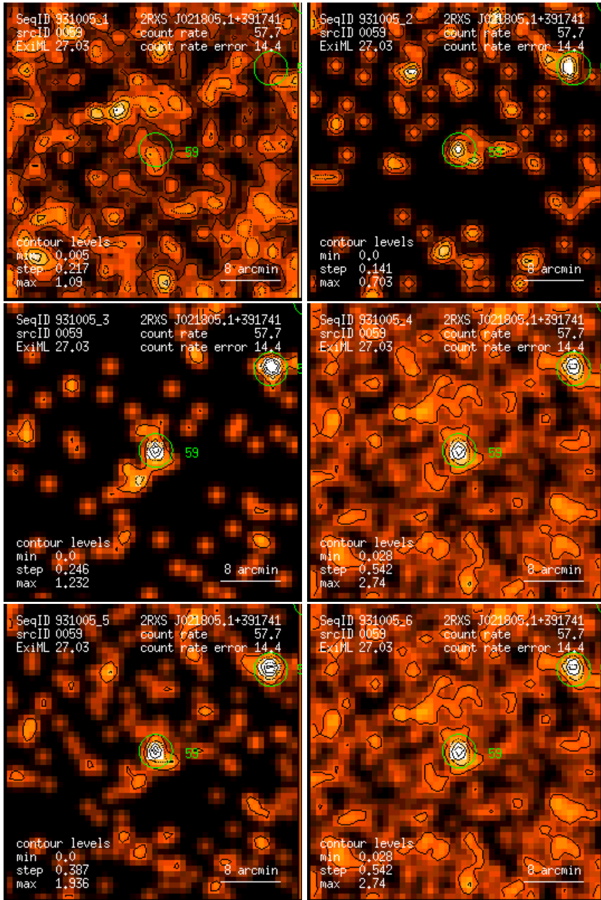
Figure 59: RASS 931005: detection 0059: band rate images, Gaussian filter: (1) PSPC channels 11 – 41, (2) 52 – 90, (3) 91 – 201, (4) 11 – 235, (5) 52 – 201, (6) 11 – 201. Broad band rates in counts/ks. Band rate contour levels in counts/ks/arcmin 2 .
