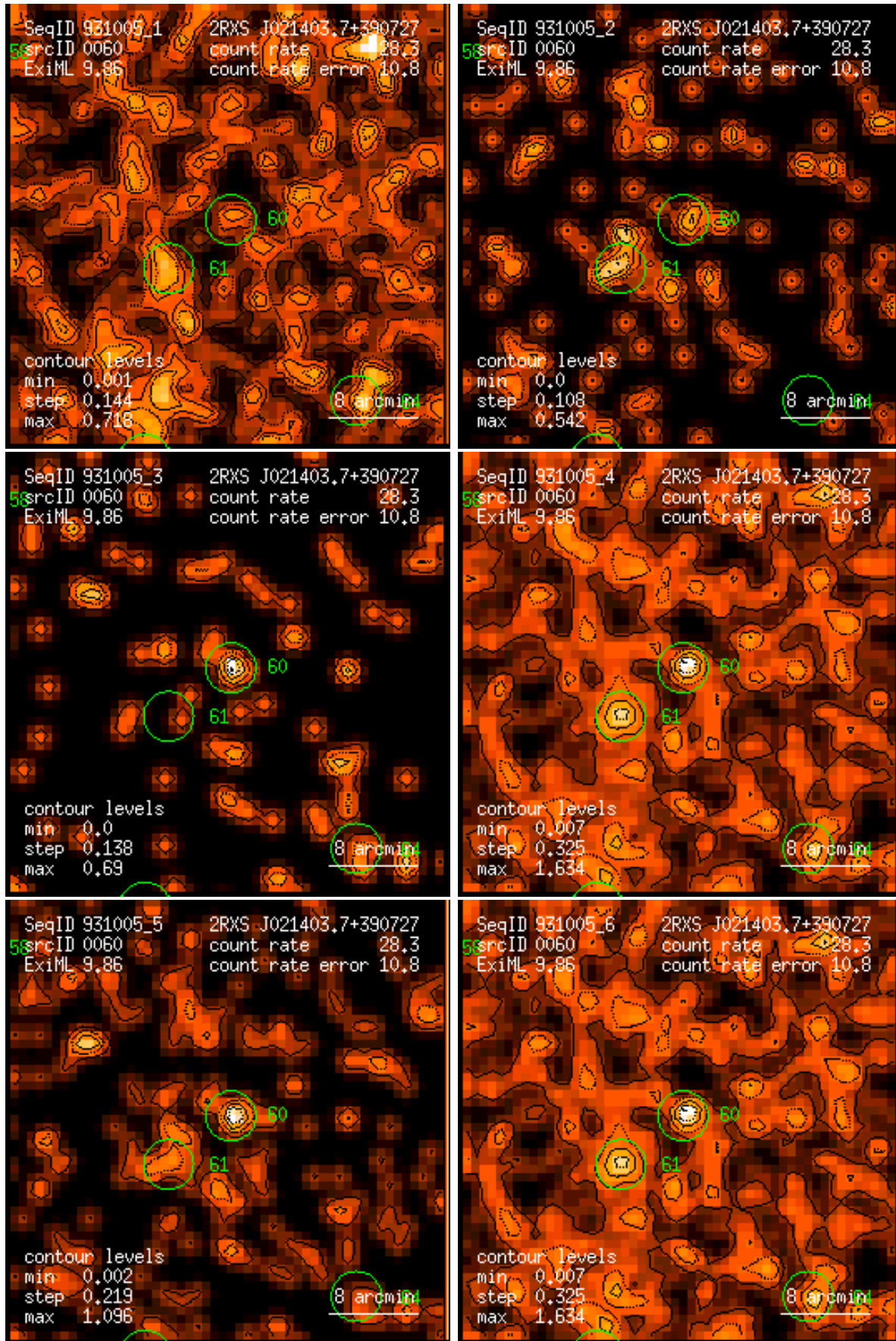
Figure 60: RASS 931005: detection 0060: band rate images, Gaussian filter: (1) PSPC channels 11 – 41, (2) 52 – 90, (3) 91 – 201, (4) 11 – 235, (5) 52 – 201, (6) 11 – 201. Broad band rates in counts/ks. Band rate contour levels in counts/ks/arcmin 2 .
