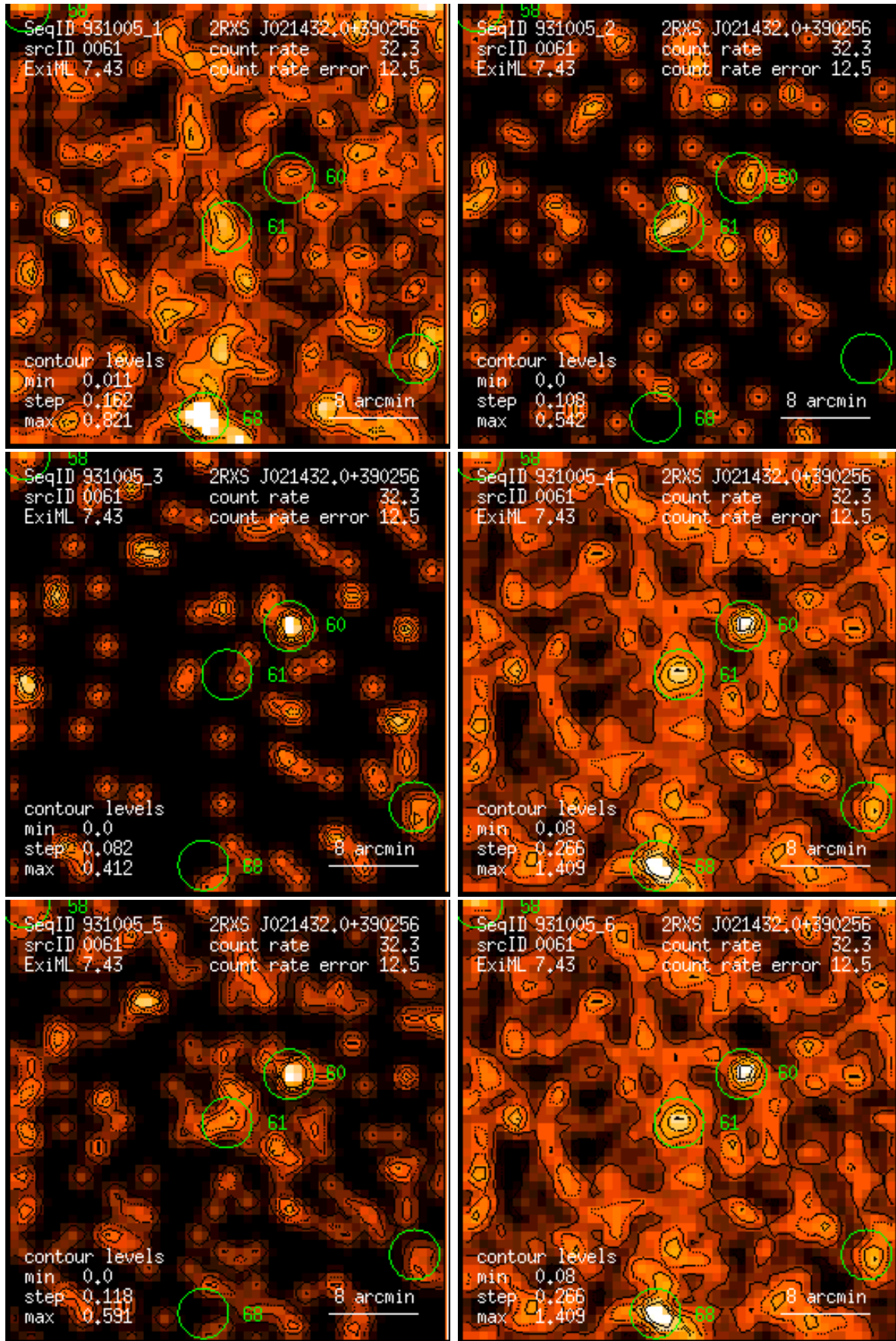
Figure 61: RASS 931005: detection 0061: band rate images, Gaussian filter: (1) PSPC channels 11 – 41, (2) 52 – 90, (3) 91 – 201, (4) 11 – 235, (5) 52 – 201, (6) 11 – 201. Broad band rates in counts/ks. Band rate contour levels in counts/ks/arcmin 2 .
