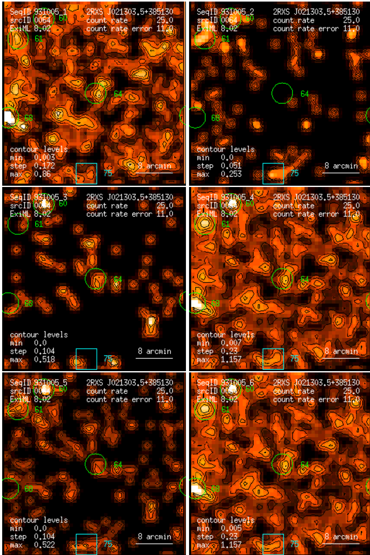
Figure 64: RASS 931005: detection 0064: band rate images, Gaussian filter: (1) PSPC channels 11 – 41, (2) 52 – 90, (3) 91 – 201, (4) 11 – 235, (5) 52 – 201, (6) 11 – 201. Broad band rates in counts/ks. Band rate contour levels in counts/ks/arcmin 2 .
